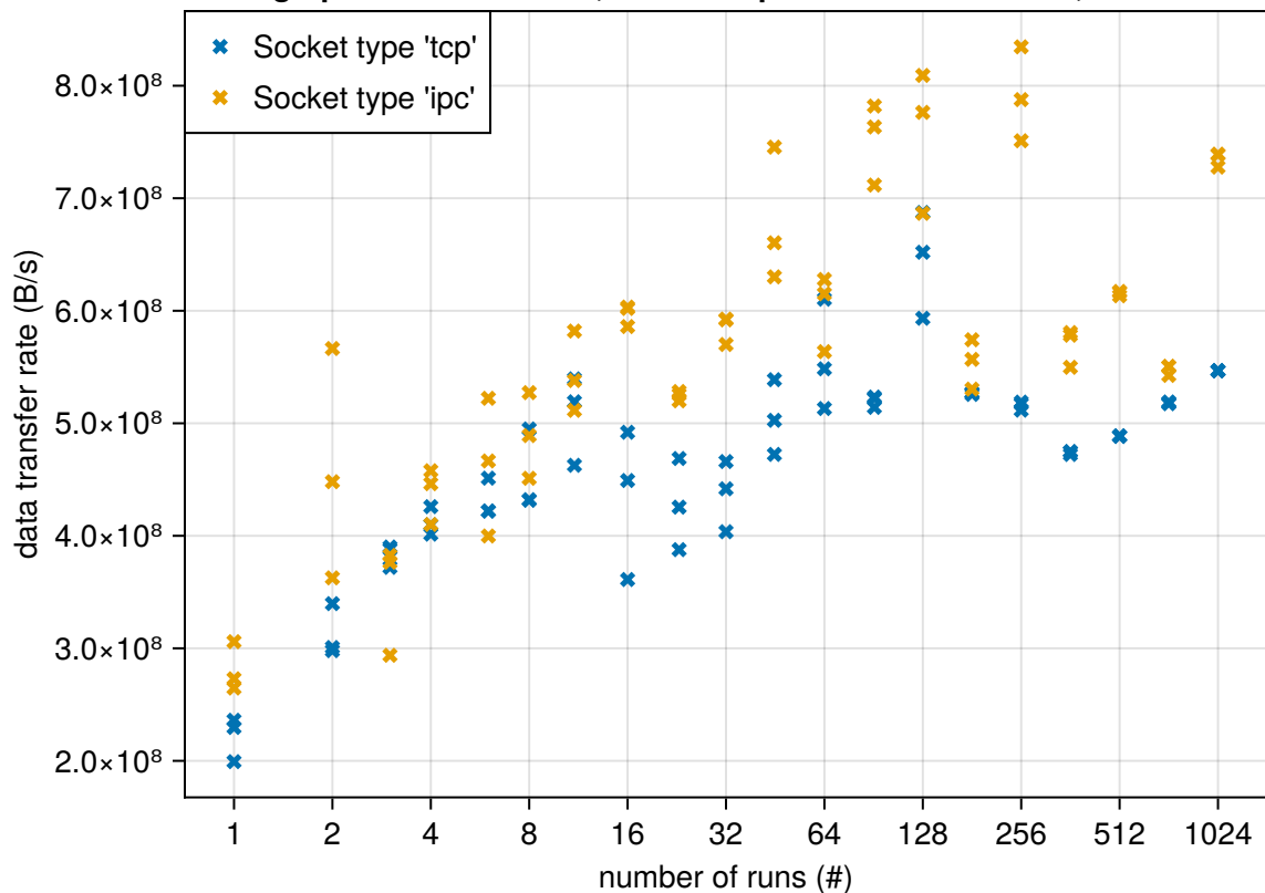
Test graph communication, sent data packet size = 32768 B, 7 transfers
