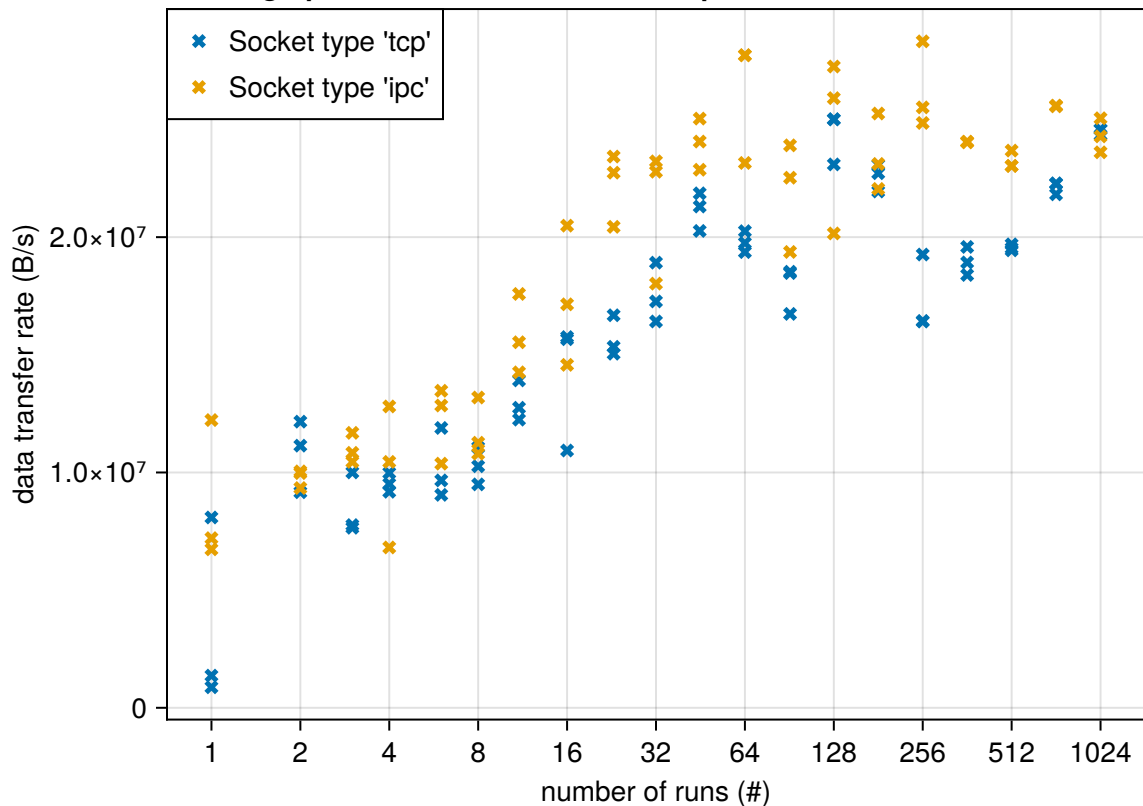
Test graph communication, sent data packet size = 512 B, 7 transfers
