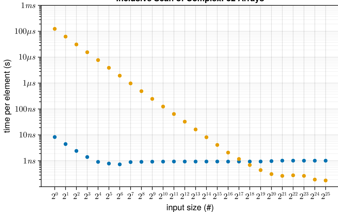
Inclusive Scan of ComplexF32 Arrays
