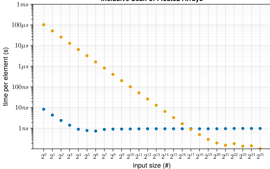
Inclusive Scan of Float32 Arrays
