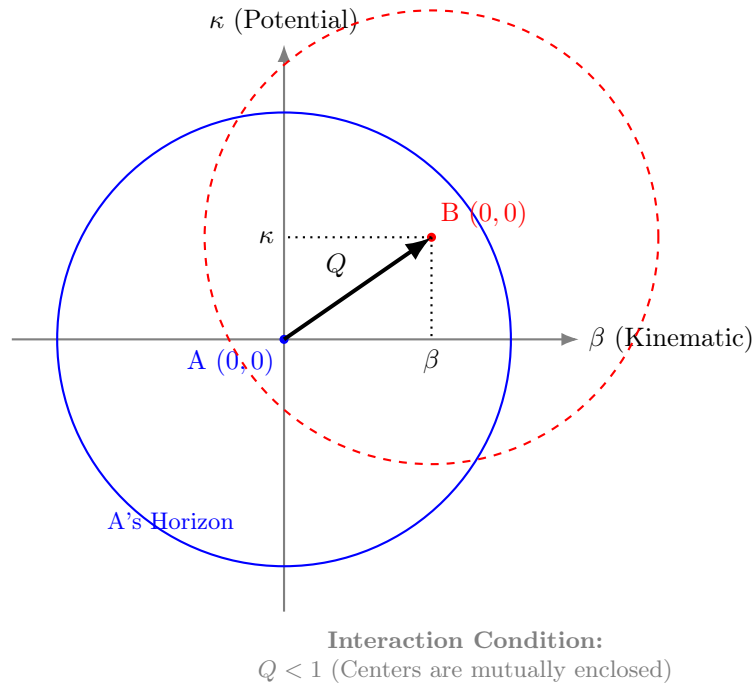
Figure 1: Relational Self-Centering. The total shift Q is defined by the amplitude projections \beta and \kappa . Interaction is causal only when the relational origin (0, 0) of B lies within A 's horizon ( Q < 1 ), ensuring mutual coverage.
