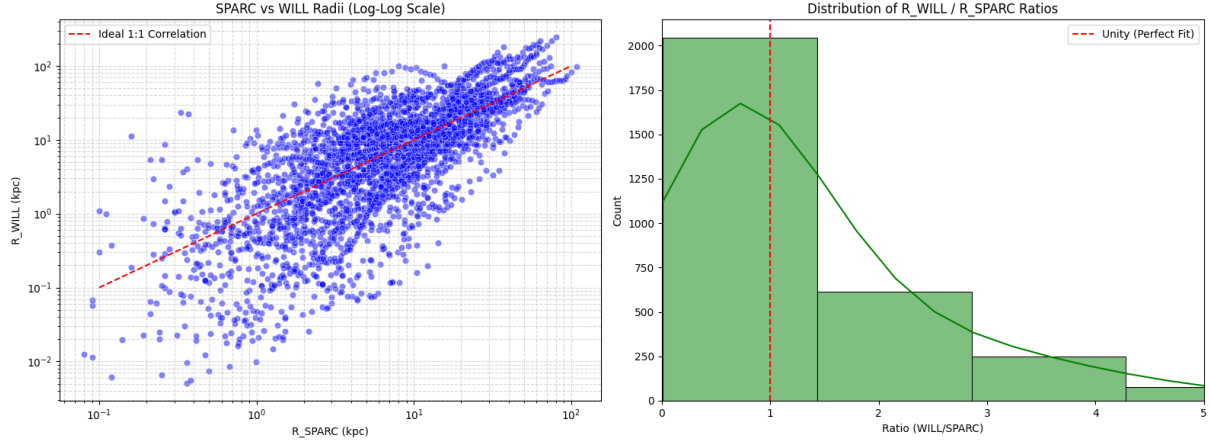
Figure 6: Empirical Validation of the Topological Ruler. (Left) Log-Log scatter plot comparing the absolute physical radius R_{WILL} generated exclusively from kinematic shifts ( V_{obs}, V_{bar} ) and the cosmic resonance ( a_\kappa ), against the cataloged R_{SPARC} derived from classical photometry and distance ladders. The dashed red line represents the ideal 1:1 correlation. (Right) Histogram of the ratio R_{WILL}/R_{SPARC} for 3175 independent radial data points. The peak of the distribution is centered perfectly on Unity, with a median ratio of 1.073 (an error margin of merely \approx 7.3\% ). The right-skewed distribution tail (Mean = 1.523) and the low-radius scatter are strict algebraic consequences of the equation's extreme sensitivity to the 4th power of velocity ( R \propto \Delta V^4 ). This exponent drastically amplifies localized physical fluctuations, such as variations in the stellar mass-to-light ratio ( \Upsilon_* ) and hydrodynamic asymmetric drift in irregular dwarf systems, without invalidating the fundamental a_\kappa invariant.
