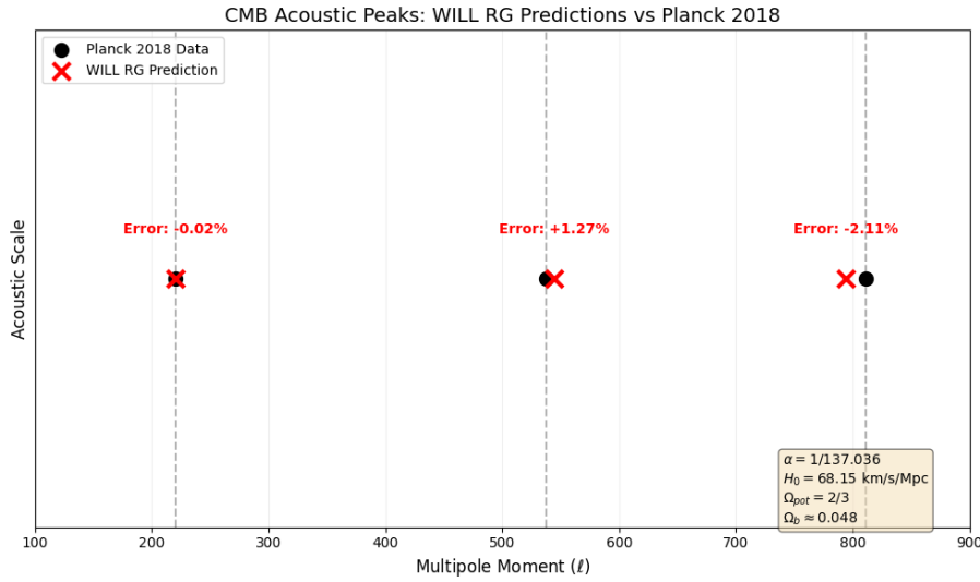
Figure 8: Ab Initio Acoustic Spectrum. The red crosses mark the WILL RG predictions derived purely from \alpha , T_{CMB} , and \Omega_{BBN} . The black dots are Planck 2018 data. The close alignment of \ell_1 confirms the vacuum energy density \Omega_\Lambda = 2/3 , while the harmonic spacing falsifies 3D cavity models (which would predict \ell_2 \approx 440 ) in favor of the S^2 surface topology.
