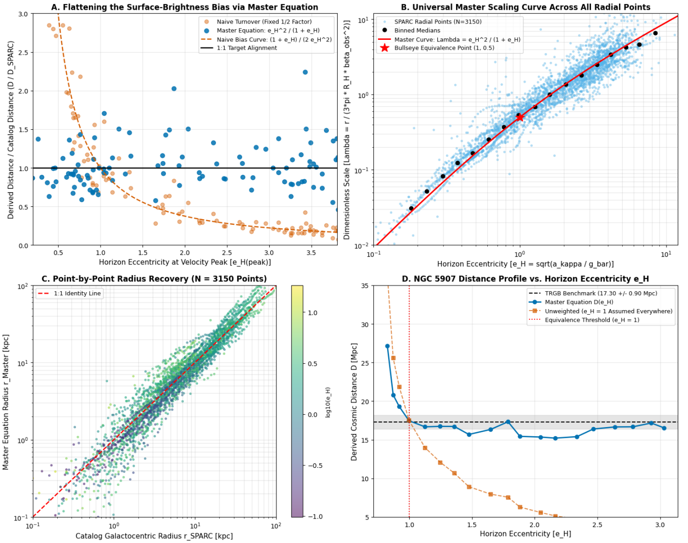
Figure 6: Verification of the Master Galactic Ladder Equation across the SPARC Database ( N = 149 Galaxies, N = 3,150 Points). Panel A: Removal of the surface-brightness bias \frac{1+e_H}{2e_H^2} (orange) via the Master Equation factor \frac{e_H^2}{1+e_H} (blue). Panel B: Collapse of all 3,150 radial points onto the dimensionless scaling curve \Lambda(e_H) = \frac{e_H^2}{1+e_H} , intersecting the Equivalence Point (1,0.5) (red star). Panel C: Point-by-point recovery of galactocentric radius r_{Master} versus r_{SPARC} across 0.1–100 kpc. Panel D: Radial distance profile of NGC 5907 versus Horizon eccentricity e_H compared to the TRGB benchmark ( 17.30 \pm 0.90 Mpc).
