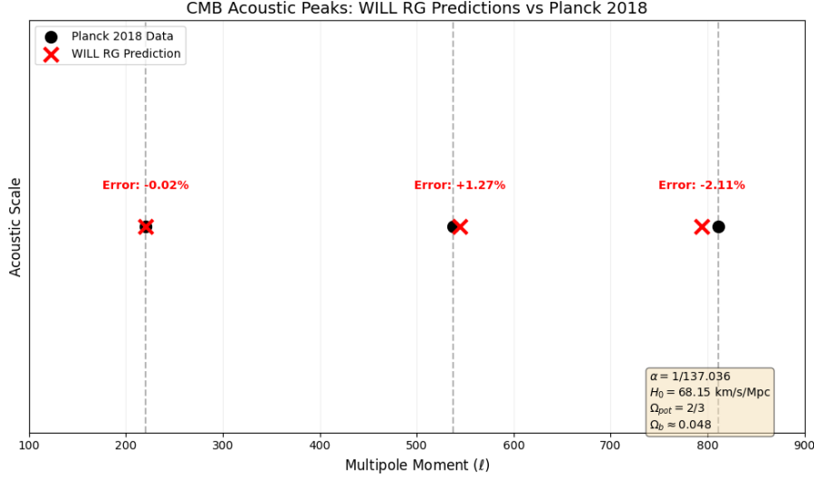
Figure 3: Ab Initio Acoustic Spectrum. The red crosses mark the WILL RG predictions derived purely from \alpha , T_{\text{CMB}} , and \Omega_{\text{BBN}} . The black dots are Planck 2018 data. The close alignment of \ell_1 confirms the vacuum energy density \Omega_\Lambda = 2/3 , while the harmonic spacing falsifies 3D cavity models (which would predict \ell_2 \approx 440 ) in favor of the S^2 surface topology.
