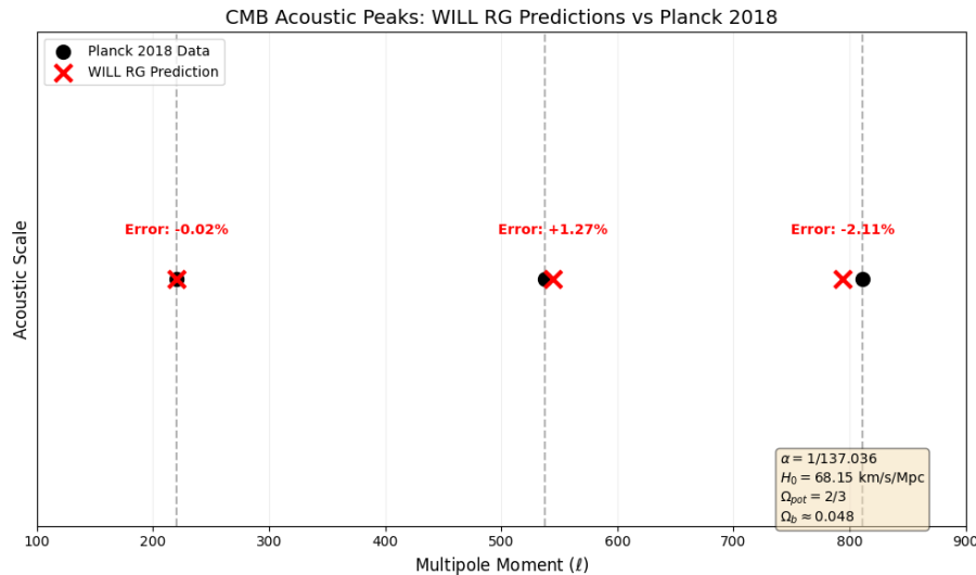
Figure 9: Ab Initio Acoustic Spectrum. The red crosses mark the WILL RG predictions derived purely from \alpha , T_{CMB} , and \Omega_{BBN} . The black dots are Planck 2018 data. The close alignment of \ell_1 confirms the vacuum energy density \Omega_\Lambda = 2/3 , while the harmonic spacing falsifies 3D cavity models (which would predict \ell_2 \approx 440 ) in favor of the S^2 surface topology.
