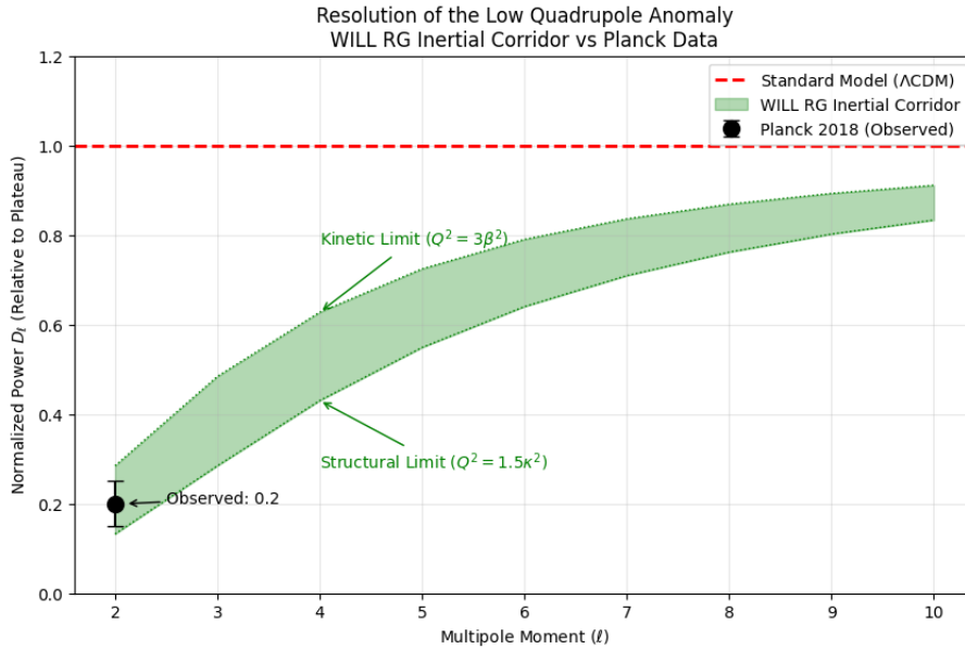
Figure 10: Resolution of the Low Quadrupole Anomaly. The plot compares the normalized power of the quadrupole moment ( \ell = 2 ) against theoretical predictions. The Standard Model ( \Lambda CDM, red dashed line) assumes a scale-invariant 3D fluid, predicting a normalized power of \approx 1.0 , which overestimates the observation by a factor of 5. WILL Relational Geometry (green shaded region) treats the Universe as a tensioned S^2 membrane, where vacuum tension acts as a high-pass filter. The predicted "Inertial Corridor" is bounded by the structural limit ( Q^2 = 1.5\kappa^2 , lower bound \approx 0.16 ) and the kinetic limit ( Q^2 = 3\beta^2 , upper bound \approx 0.32 ). The Planck 2018 observation ( D_{\ell=2} \approx 0.20 , black point) falls within the WILL RG corridor, confirming the geometric suppression of large-scale modes due to vacuum tension.
