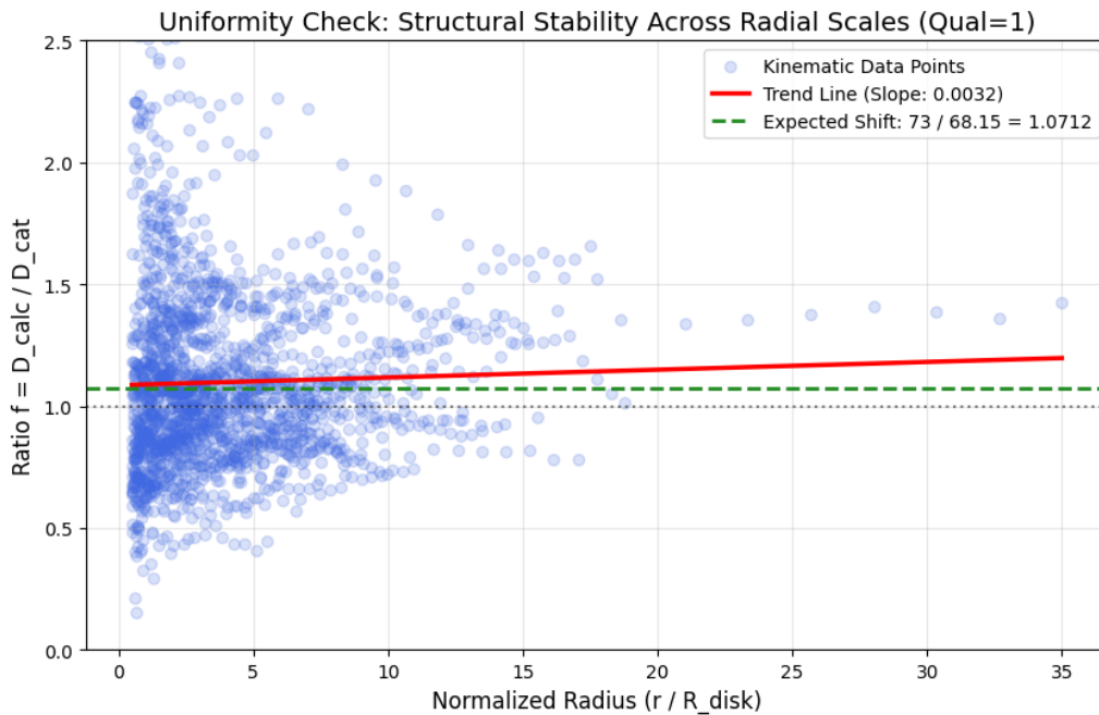
Figure 7: Structural Stability Across Radial Scales. The ratio f = D_{calc}/D_{cat} evaluated as a continuous function of normalized galactic radius ( r/R_{disk} ). The solid red line represents the linear trend, which is statistically indistinguishable from zero (Slope: 0.00318, p-value: 0.182). The calculated ratio exhibits structural flatness from the inner disk to the kinematic periphery, proving that the geometric transition from Newtonian dominance ( V_{bar}^2 ) to Resonant dominance ( \sqrt{V_{bar}^2 R a_{\kappa}} ) operates without cumulative error.
