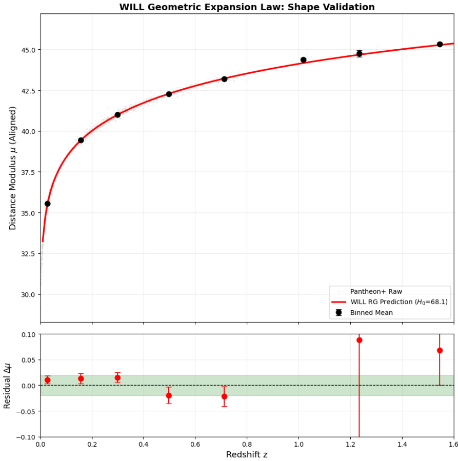
Figure 8: Ab Initio Prediction of Cosmic Expansion. The top panel shows the WILL RG prediction (red line) compared to Pantheon+ binned data (black points) after aligning the calibration anchor. The bottom panel displays the residuals. The curve is not a fit; it is generated purely from microphysics ( T_{CMB}, \alpha ) and geometric partitioning ( \Omega = 1/3, 2/3 ).
