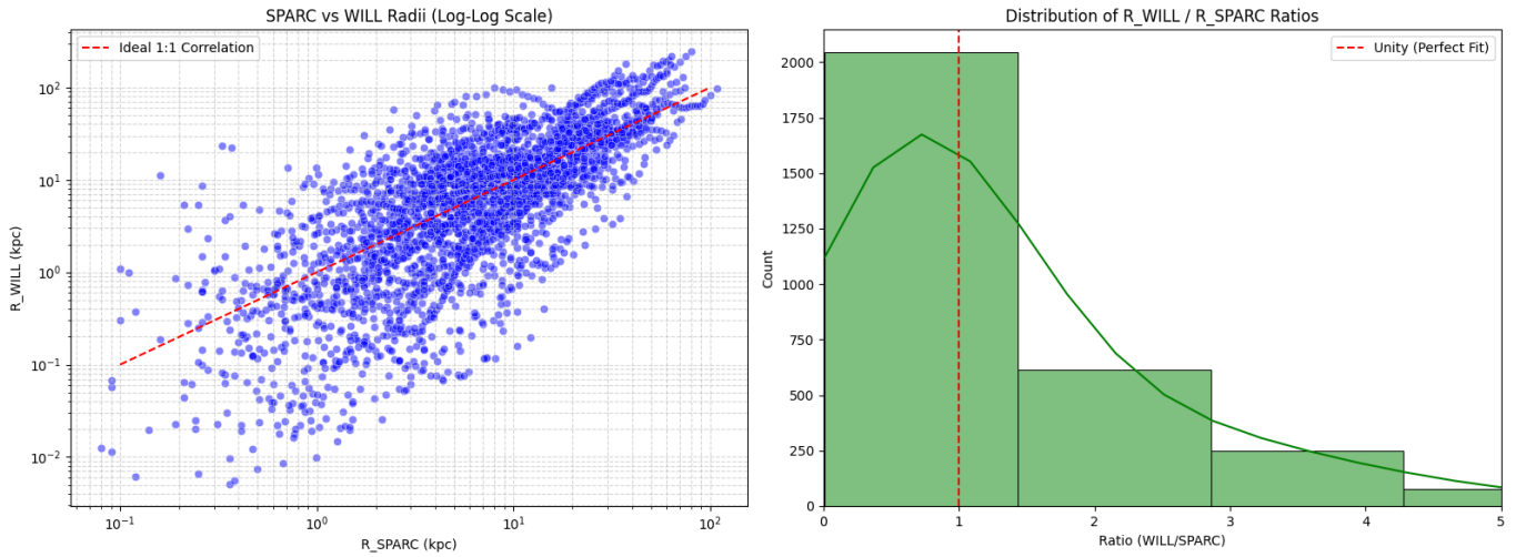
Figure 6: Empirical Validation of the Topological Ruler. (Left) Log-Log scatter plot comparing the absolute physical radius R_{WILL} generated exclusively from kinematic shifts ( V_{obs} , V_{bar} ) and the cosmic resonance ( a_\kappa ), against the cataloged R_{SPARC} derived from classical photometry and distance ladders. The dashed red line represents the ideal 1:1 correlation. (Right) Histogram of the ratio R_{WILL}/R_{SPARC} for 3175 independent radial data points. The peak of the distribution is centered perfectly on Unity, with a median ratio of 1.073 (an error margin of merely \approx 7.3\% ). The right-skewed distribution tail (Mean = 1.523) and the low-radius scatter are strict algebraic consequences of the equation's extreme sensitivity to the 4th power of velocity ( R \propto \Delta V^4 ). This exponent drastically amplifies localized physical fluctuations, such as variations in the stellar mass-to-light ratio ( \Upsilon_* ) and hydrodynamic asymmetric drift in irregular dwarf systems, without invalidating the fundamental a_\kappa invariant.
