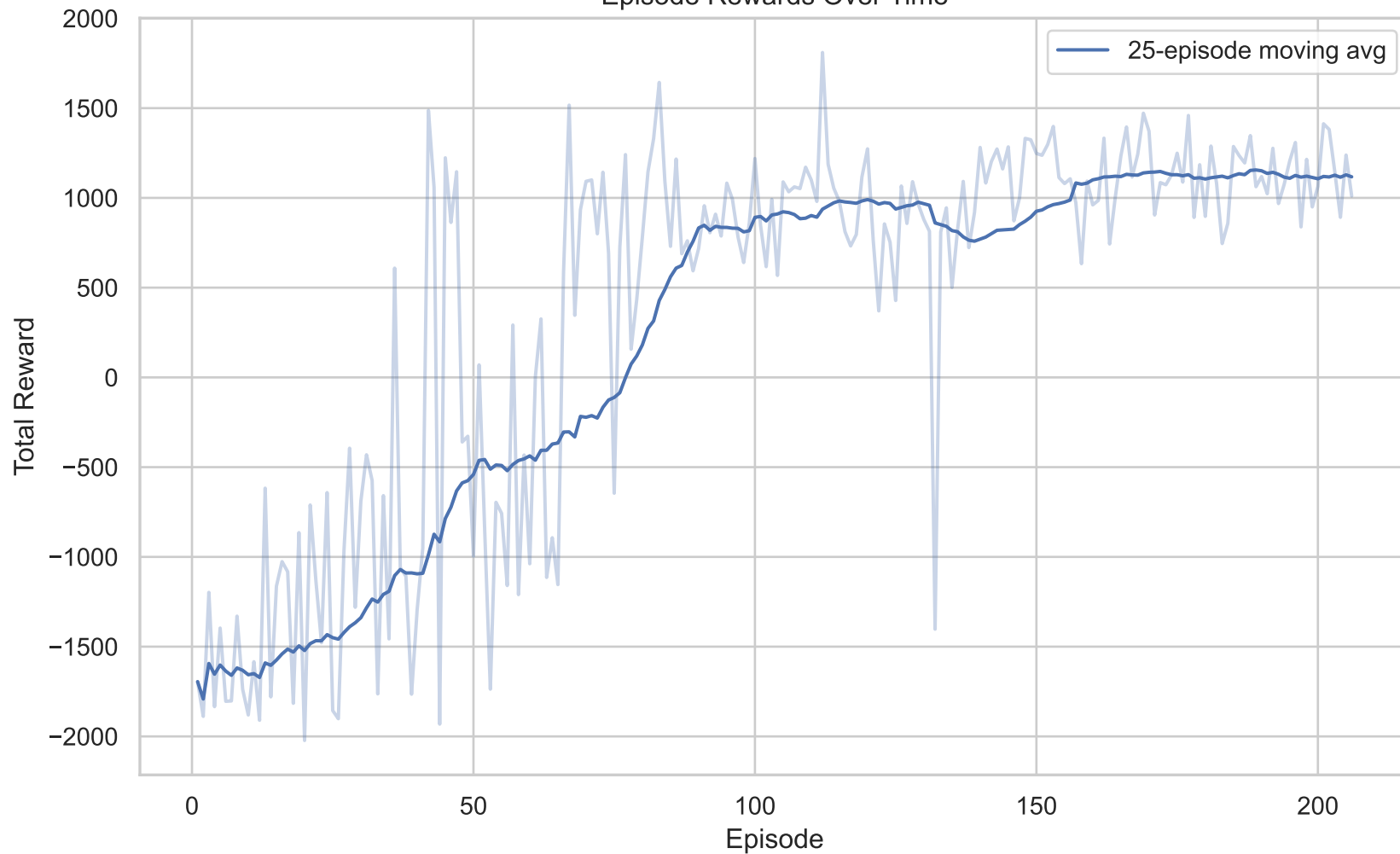
Episode Rewards Over Time
