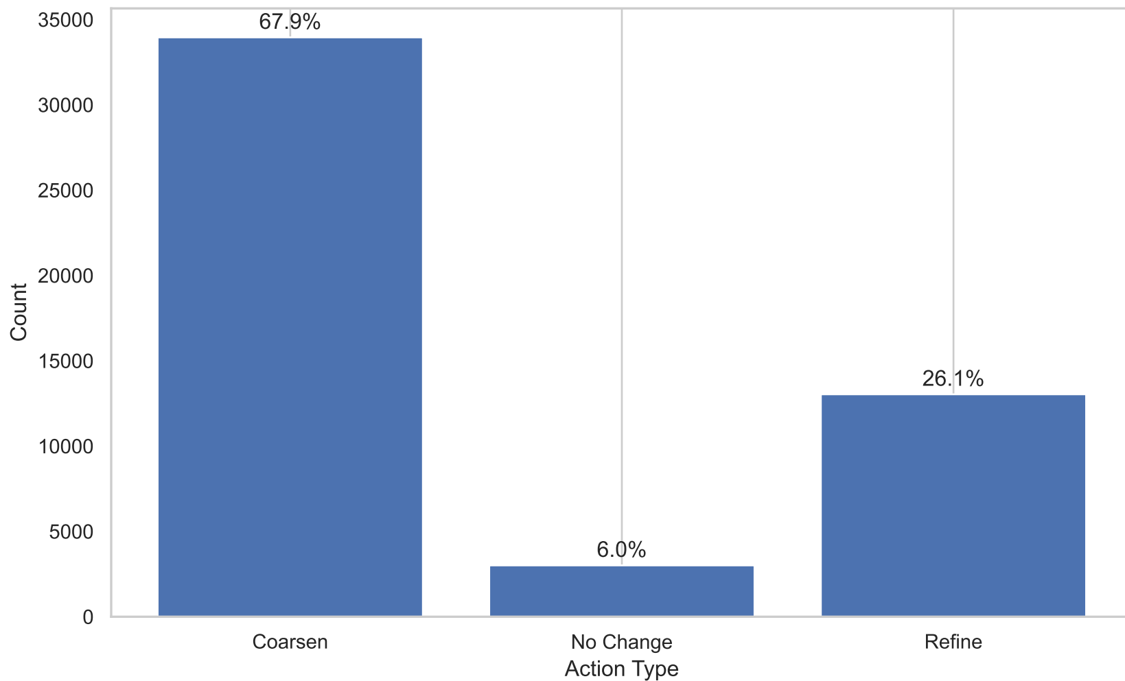
Action Distribution
