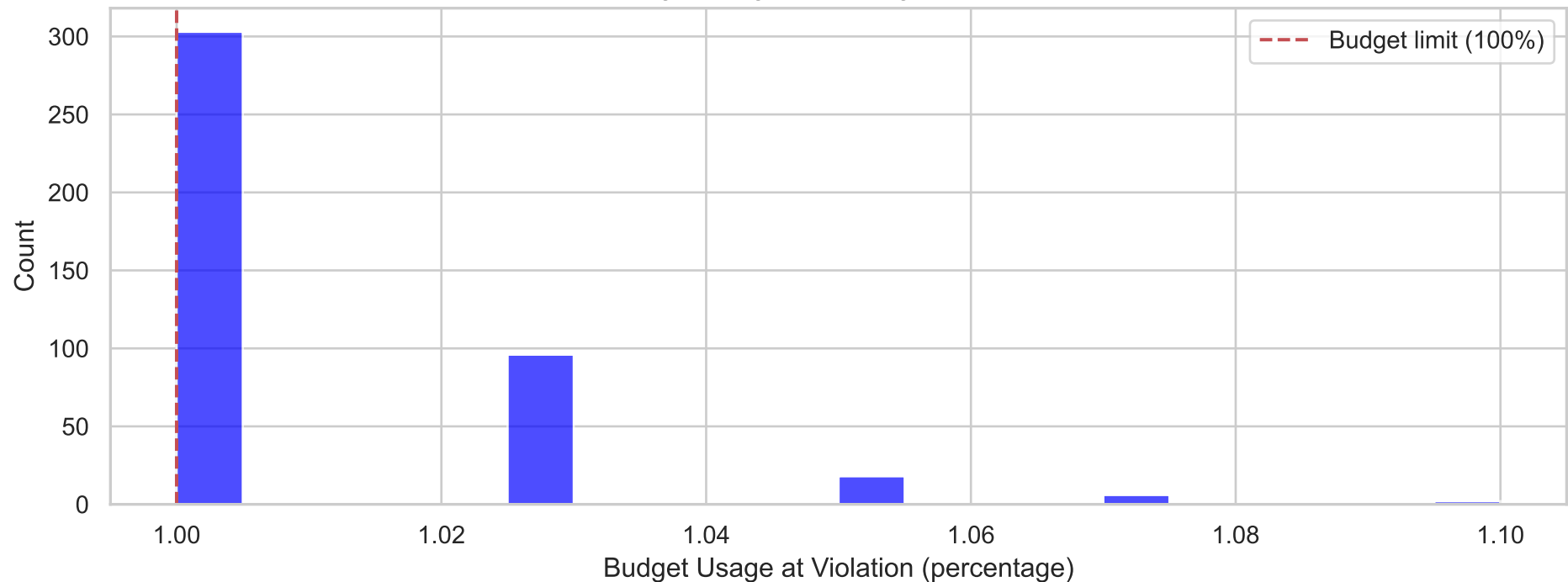
Budget Usage Percentage at Violation
