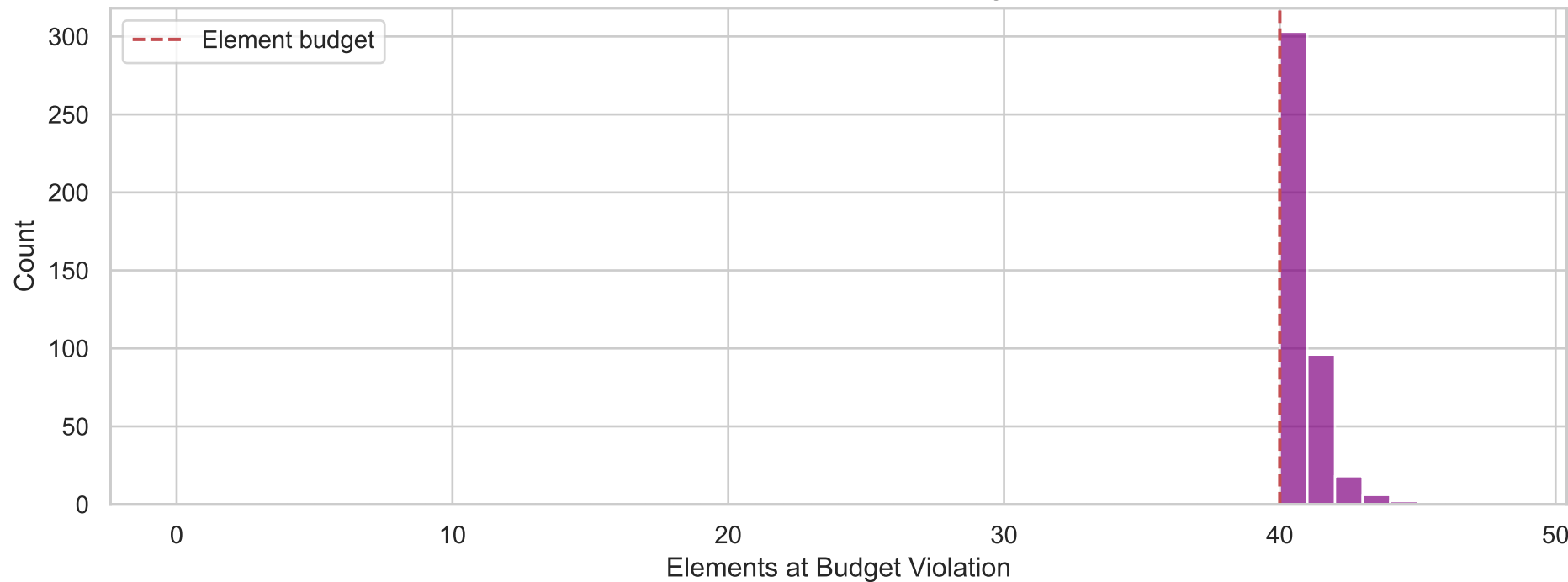
Distribution of Element Counts at Budget Violation
