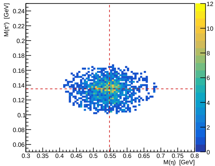
gate BDT
