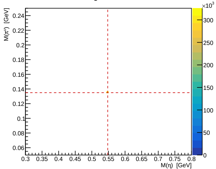
gate BDT
