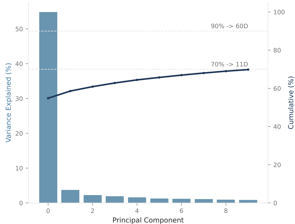
(a) Refusal Space Dimensionality
