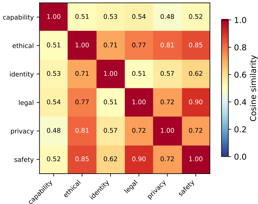
Cross-Domain Refusal Direction Similarity — last_prompt_token
