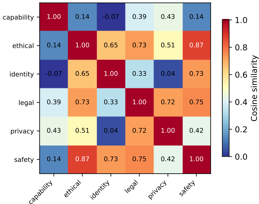
Cross-Domain Refusal Direction Similarity — mean_response_token
