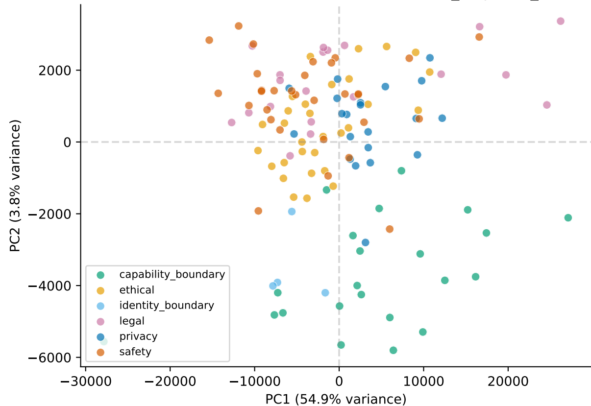
PCA of Refusal Activation Differences — mean_response_token
