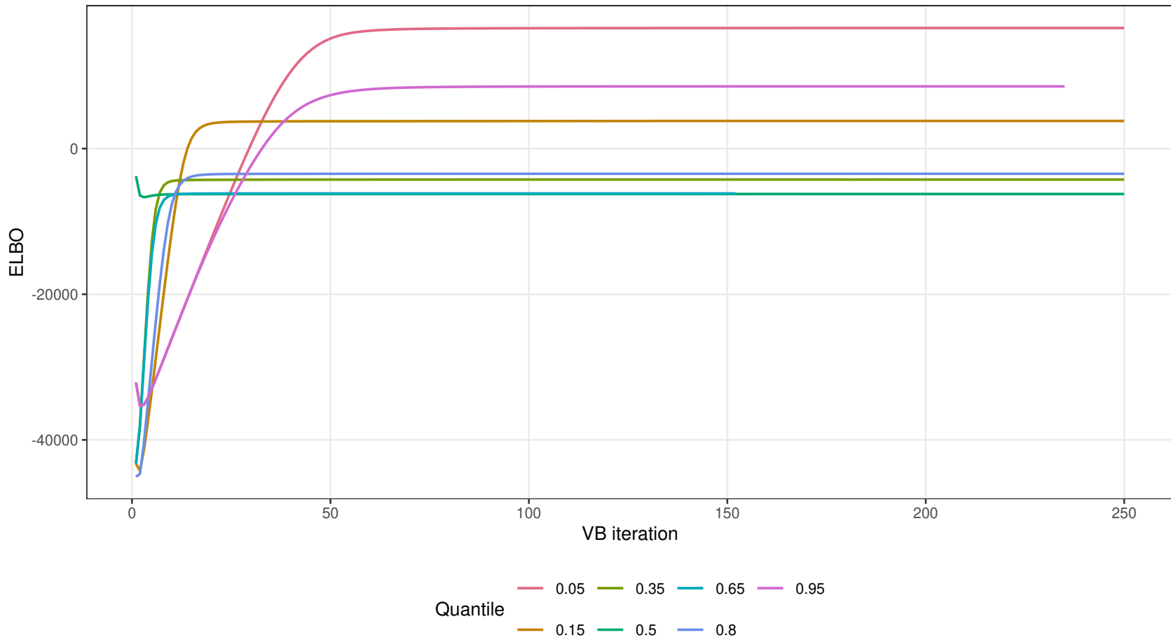
VB ELBO Traces Across Quantile Fits
