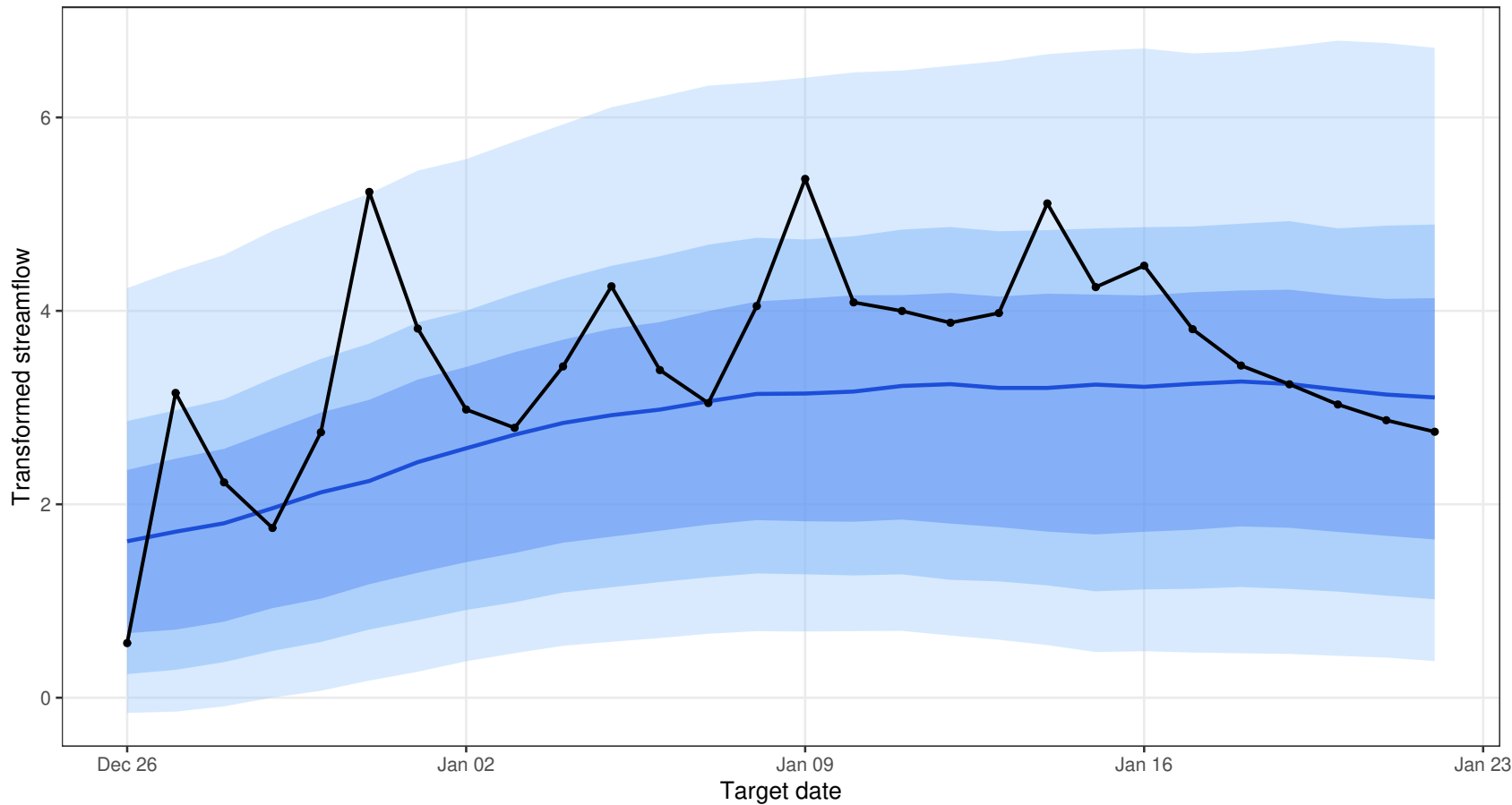
Q-DESN Synthesized Predictive Quantile Bands
