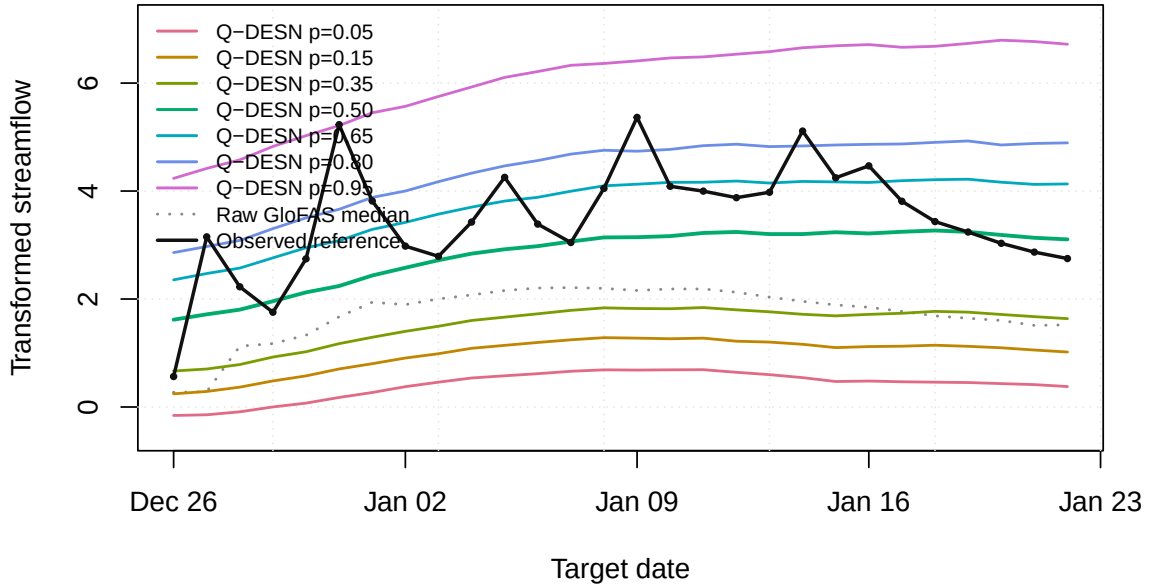
Figure 2: Raw GloFAS quantile paths, discrepancy-corrected Q-DESN quantile paths after monotone synthesis and synthesis-time spread calibration, and held-out reference streamflow over the issued forecast window for the selected GloFAS application run.
