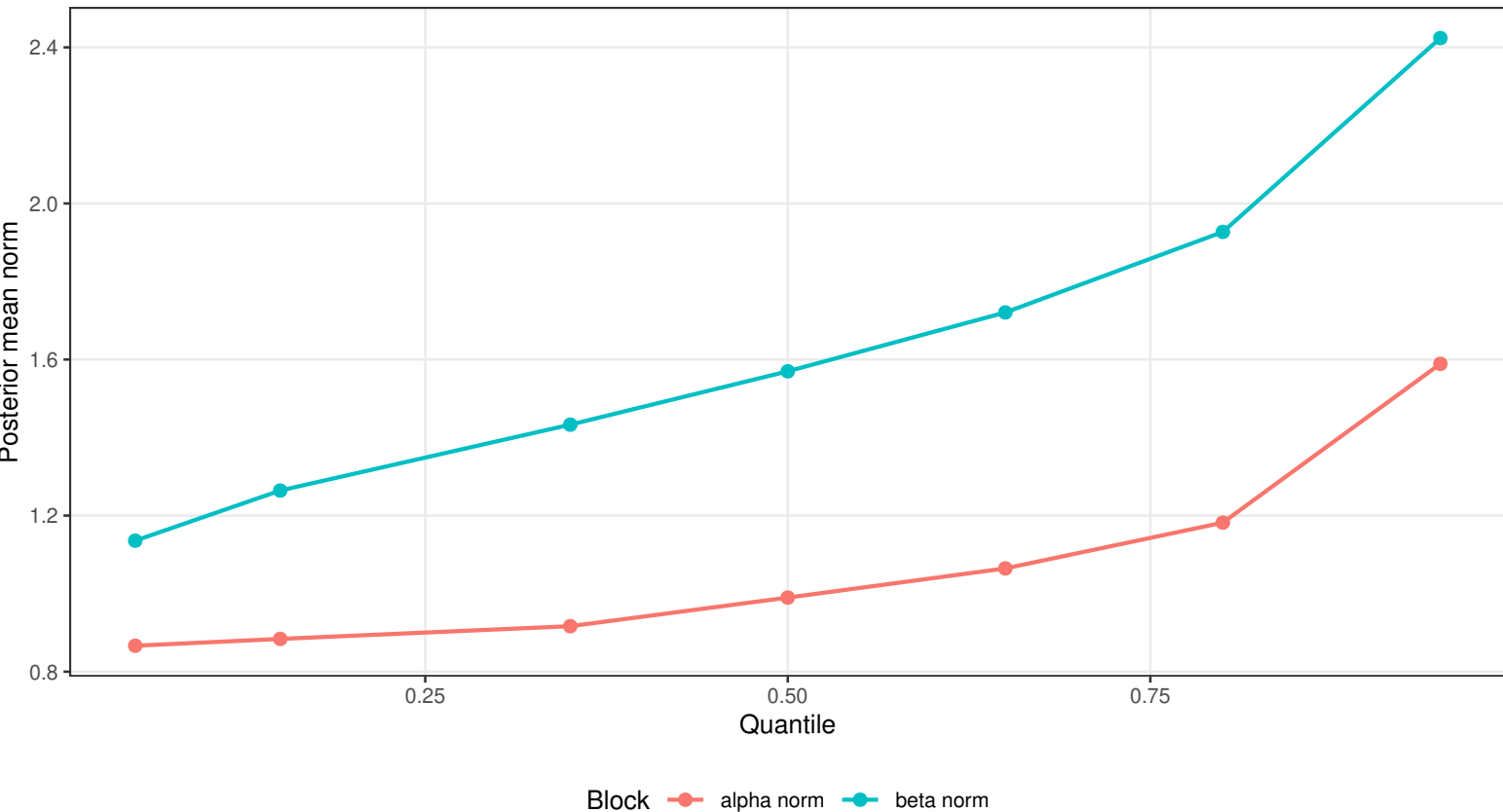
Posterior Readout-Norm Summaries by Quantile
