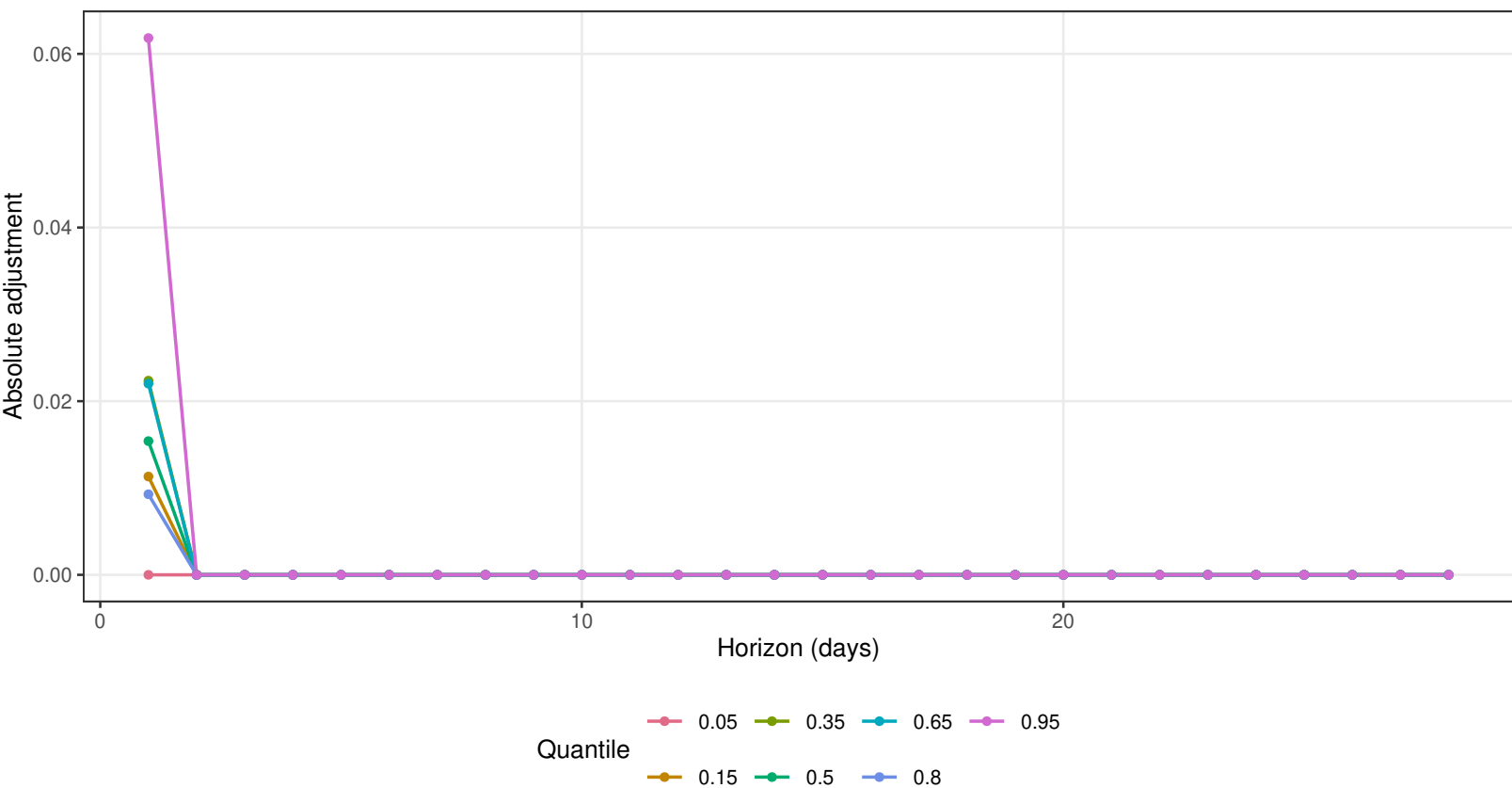
Post-Hoc Monotone Synthesis Adjustment for Q-DESN
