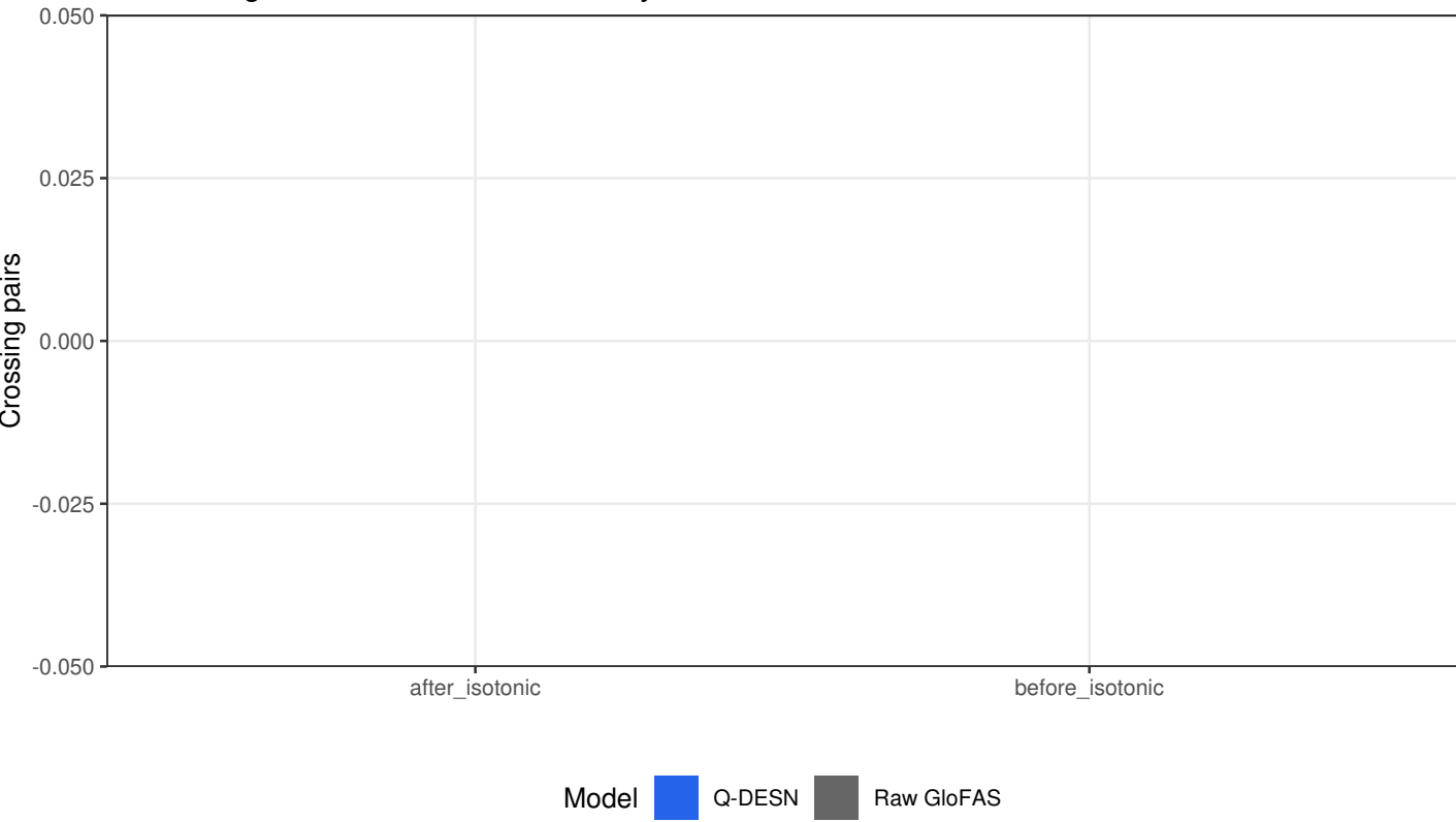
Quantile Crossing Count Before and After Synthesis
