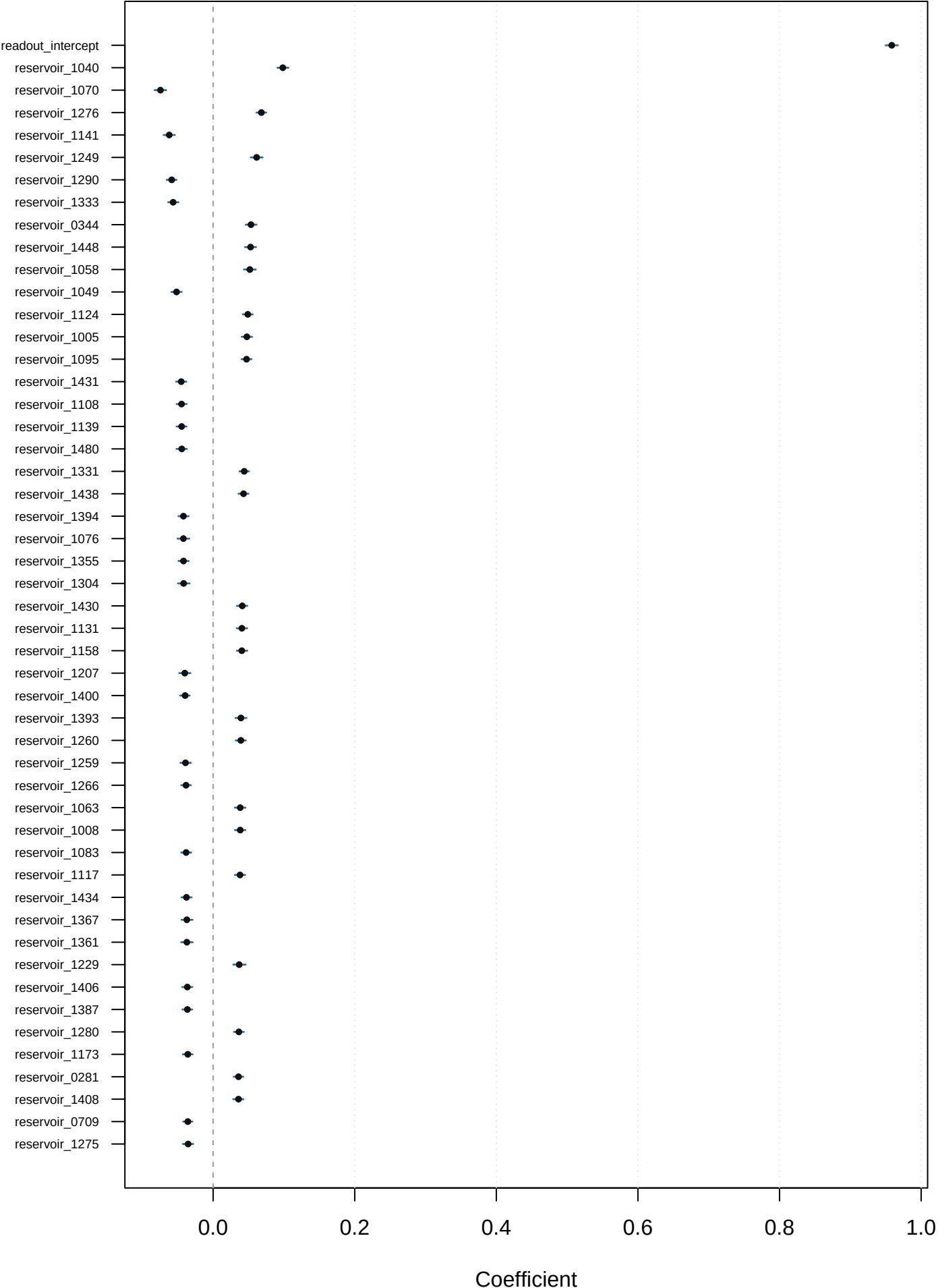
Shared-quantile readout coefficients, p=0.5
