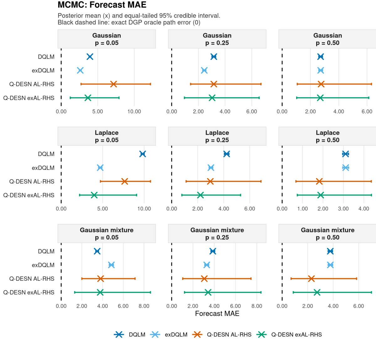
Figure 1: MCMC posterior uncertainty for forecast MAE in the single-quantile simulation. Horizontal segments show equal-tailed 95% posterior intervals and crosses show posterior means. Each panel has its own horizontal scale; lower is better. The dashed line marks the exact DGP value of zero for quantile-path error. Intervals condition on the simulated series, evaluation design, and case-specific selected specification.
