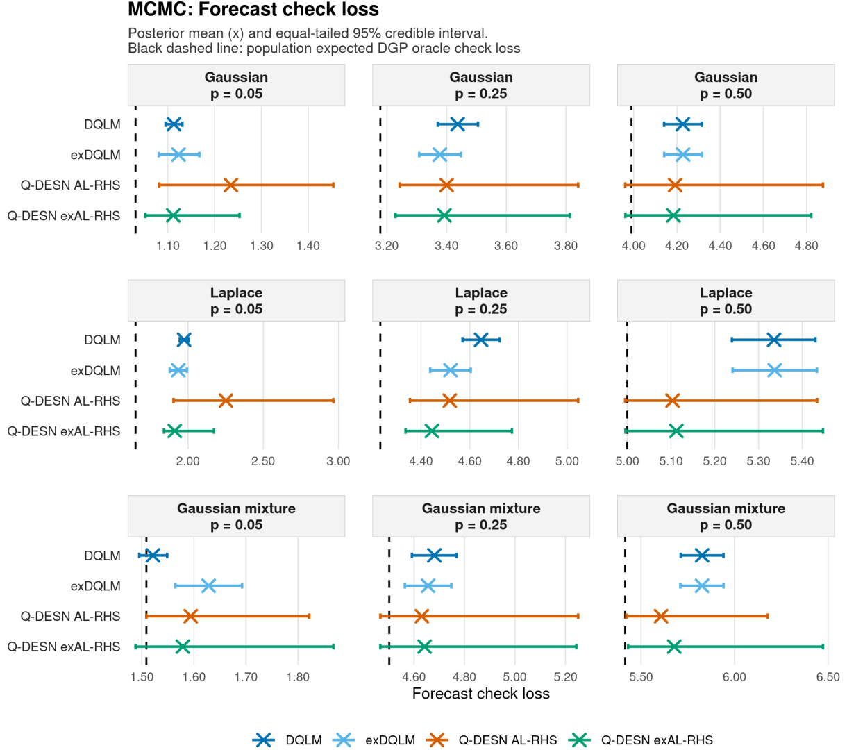
Figure 2: MCMC posterior uncertainty for forecast check loss in the single-quantile simulation. Horizontal segments show equal-tailed 95% posterior intervals and crosses show posterior means. Each panel has its own horizontal scale; lower is better. The dashed line marks population expected check loss at the true conditional quantile. Conditional finite-sample intervals may cross this reference.
