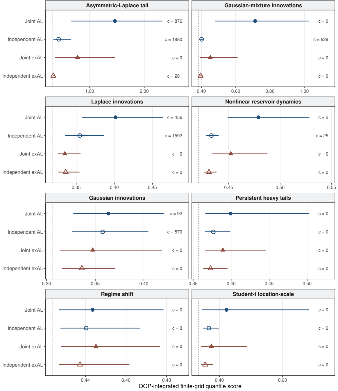
Figure 3: Posterior DGP-integrated finite-grid quantile scores under the shared-backbone design. Points are posterior means and horizontal bars are equal-tailed 95% intervals; lower is better. Dashed lines mark the oracle finite-grid score. Filled symbols denote joint fits and open symbols independent fits; blue denotes AL and red exAL. Labels c give raw crossings in the posterior-mean forecast grid; all counts after rearrangement are zero.
