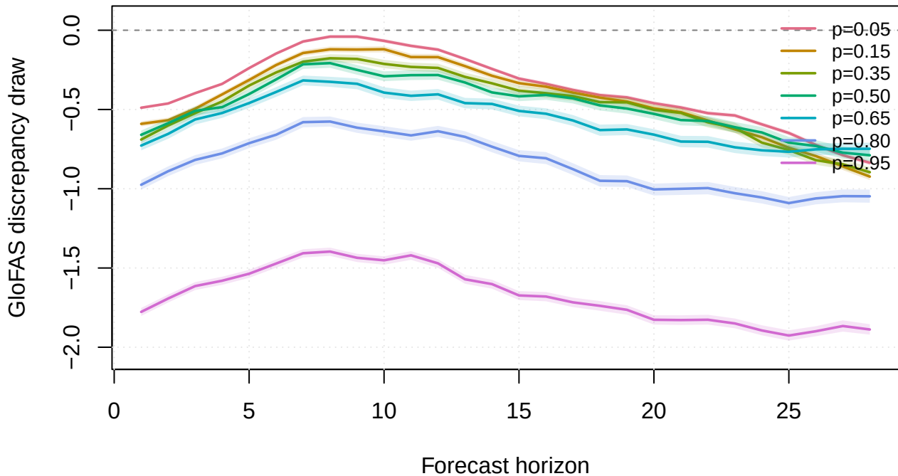
Discrepancy posterior draws by horizon
