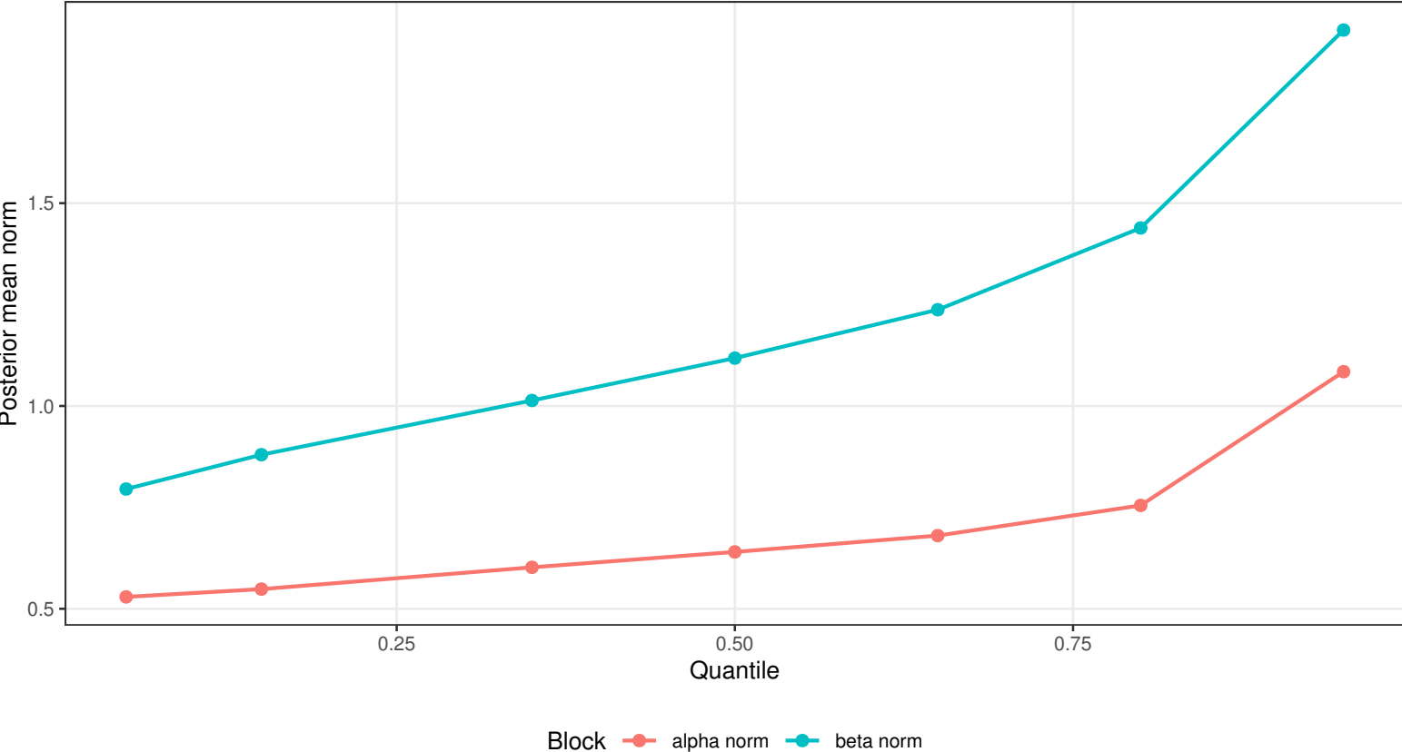
Posterior Readout-Norm Summaries by Quantile
