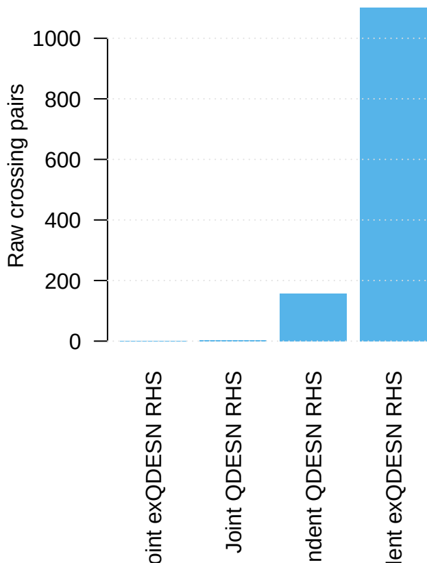
Raw crossings
