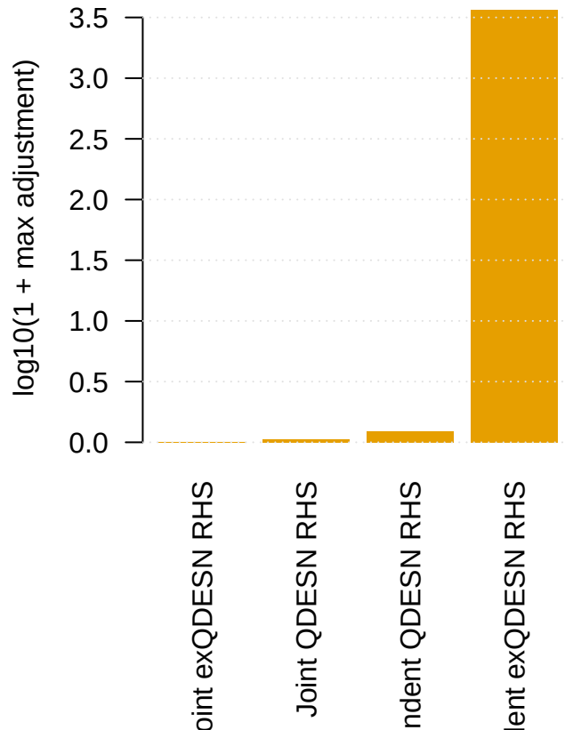
Monotone adjustment
