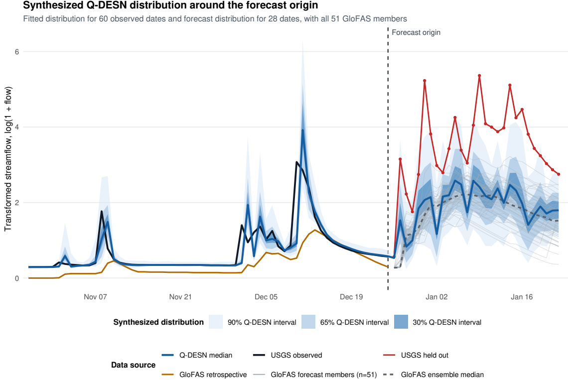
Figure 4: Synthesized Q-DESN readout bands for the GloFAS retrospective reference case over the final 60 observed dates and the subsequent 28-day forecast window. The nested blue bands are the 90%, 65%, and 30% quantile intervals, and the blue path is the median. The vertical dashed line marks the forecast origin. Black and red paths denote observed and held-out USGS streamflow, respectively; orange denotes retrospective GloFAS, and thin gray paths show all 51 issued GloFAS ensemble members, with their median dashed. Forecast scores use the post-origin targets in Table 9.
