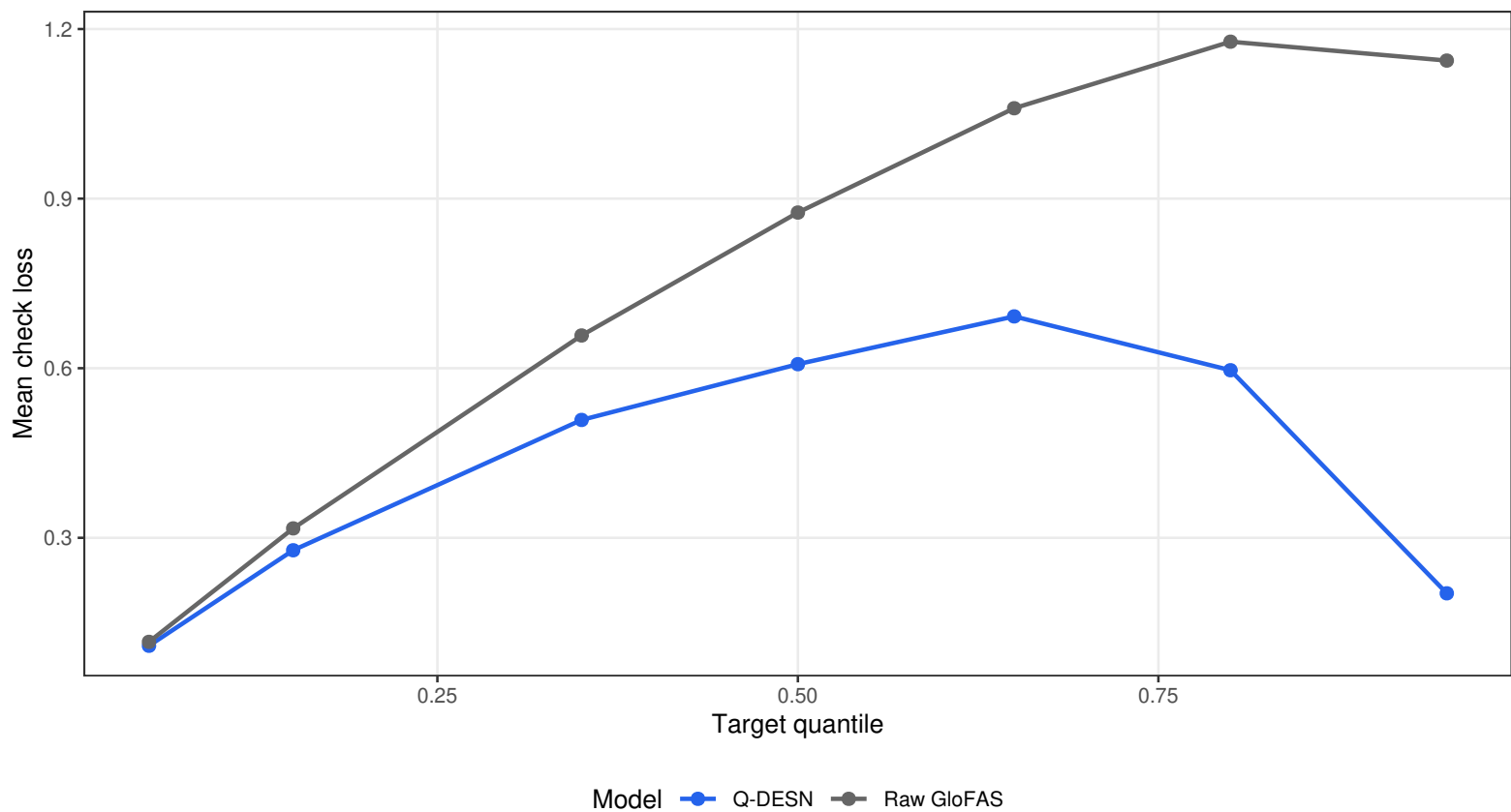
Mean Check Loss by Target Quantile
