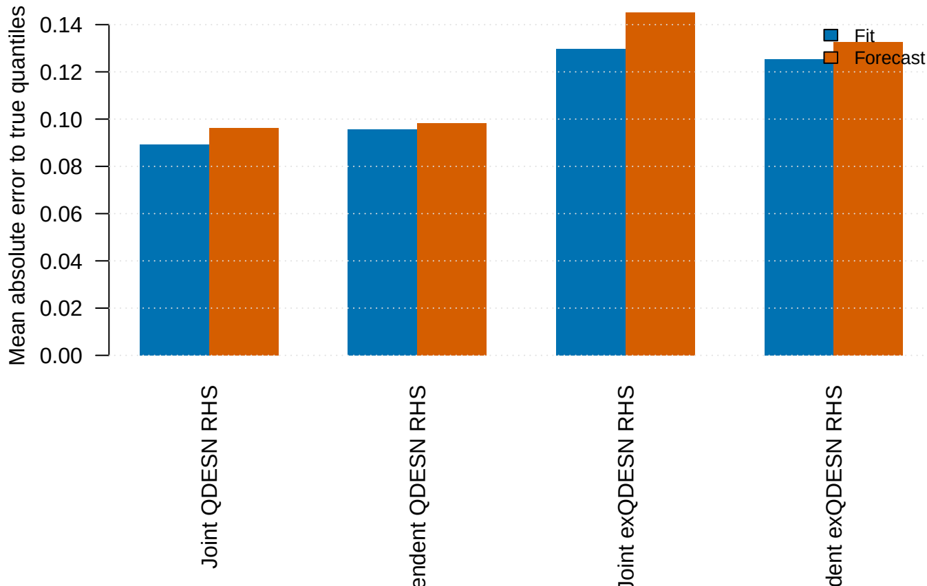
VB fit and forecast truth error
