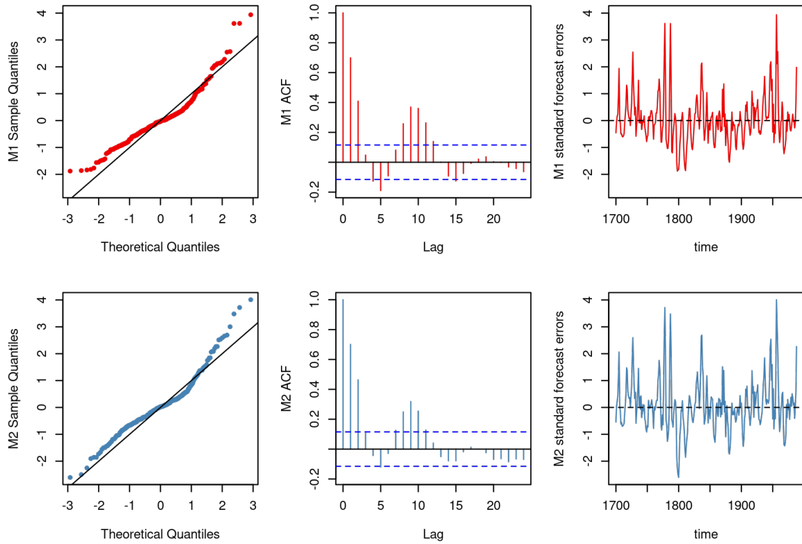
Figure 4: Example 2: Sunspots. The QQ plots (left column), ACF plots of the PIT sequence (center column), and MAP one-step-ahead standardized forecast errors (right column) from the DQLM (red) and exDQLM (blue).
