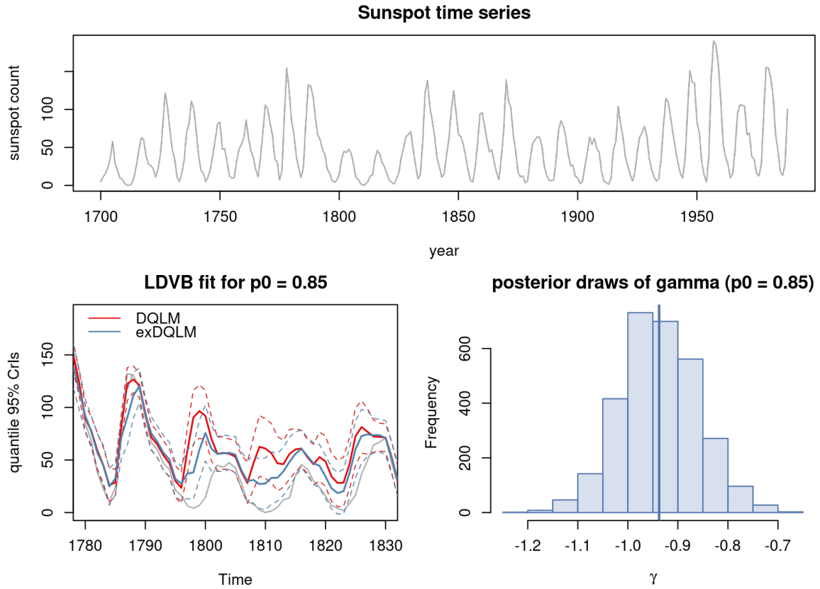
Figure 3: Example 2: Sunspots. Top: The sunspot time series from 1700 to 1988. Bottom left: posterior mean estimates and 95% CrIs of the estimated quantiles from the DQLM (red) and exDQLM (blue), plotted with the data (grey) from 1780 to 1830. Bottom right: Histogram of samples from the approximated posterior distribution of \gamma under the exDQLM.
