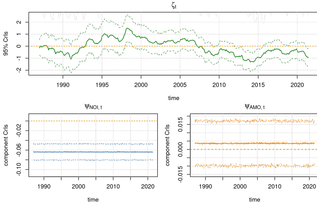
Figure 7: Example 3: Big Tree water flow. Posterior mean estimates and 95% CrIs of the transfer-function states in MTF. The top panel shows the accumulated transfer effect \zeta_t . The bottom panels show the instantaneous transfer coefficients \psi_{\text{NOI},t} and \psi_{\text{AMO},t} , which are static here because their discount factors are set to 1. Horizontal dotted orange lines mark zero.
