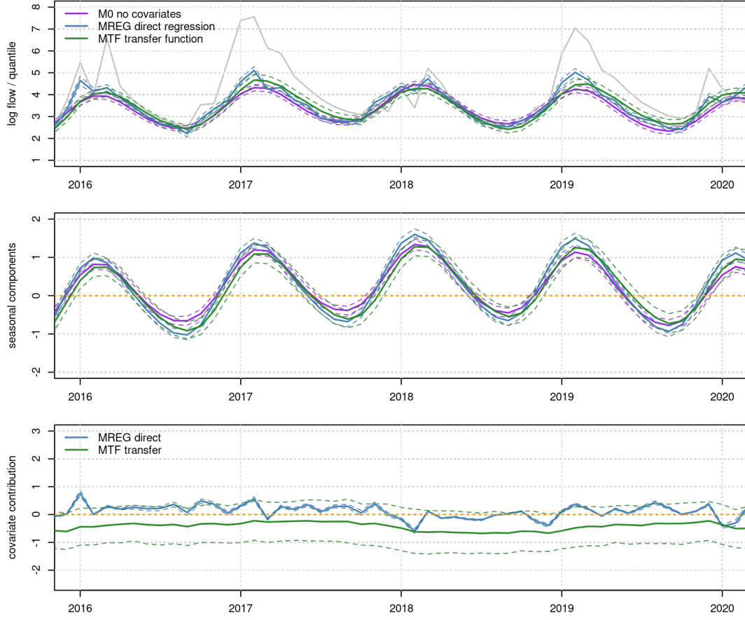
Figure 6: Example 3: Big Tree water flow. Top: posterior mean estimates and 95% CrIs of the fitted 0.15 quantile from the no-covariate baseline M0 (purple), direct-regression model MREG (blue), and transfer-function model MTF (green), plotted with the data (grey) from 2016 to 2020. Middle: posterior mean estimates and 95% CrIs of the combined seasonal components implied by the annual, semiannual, and low-frequency harmonics. Bottom: posterior mean estimates and 95% CrIs of the direct-regression contribution in MREG and the transfer-function contribution in MTF. The horizontal orange dotted lines are at zero for reference.
