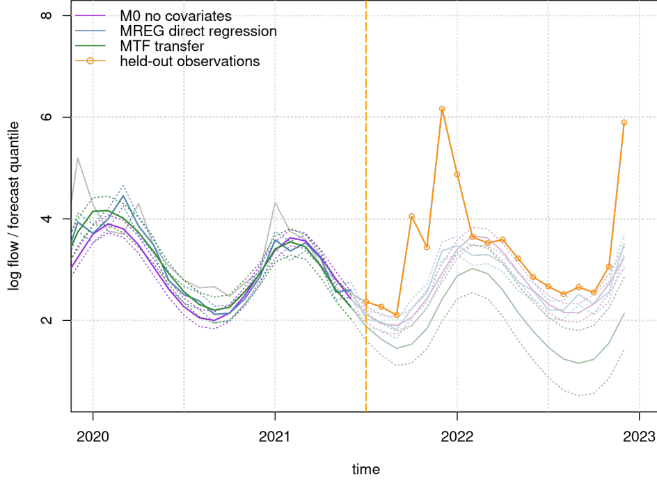
Figure 8: Example 3: Big Tree water flow. Held-out 18-month conditional forecast display from July 2021 through December 2022. The vertical dot-dashed line marks the forecast origin after the final training month, June 2021. Solid lines indicate posterior mean forecast quantiles and dotted lines indicate pointwise 95% CrIs for M0, MREG, and MTF. Held-out observations are shown as orange circles. The forecasts are conditional on the observed holdout-period NOI and AMO values.
