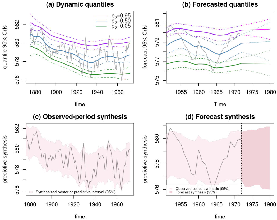
Figure 2: Example 1: Lake Huron. Top-left: posterior mean estimates and 95% CrIs of the estimated quantiles, plotted with the data (grey). Top-right: forecasted quantile estimates and 95% credible intervals (seen after 1972), along with the filtered quantile estimates and 95% credible intervals (seen from 1952 to 1972). Bottom-left: synthesized posterior predictive 95% interval over the observed period. Bottom-right: observed-period synthesis near the forecast origin (lighter band) and synthesized posterior predictive 95% interval over the eight-step forecast window (slightly darker rose band); the vertical dotted line marks the forecast origin.
