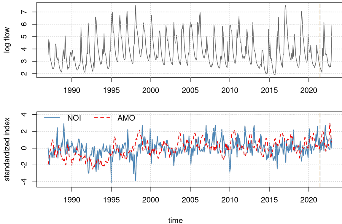
Figure 5: Example 3: Big Tree water flow. Top: observed average monthly water flow at the Big Tree gauge of the San Lorenzo River in Santa Cruz County, CA, plotted on the log scale. Bottom: standardized monthly values of the Northern Oscillation Index (NOI) and Atlantic Multidecadal Oscillation (AMO) index. The displayed modeling window spans January 1987 through December 2022, and the vertical dashed line marks the beginning of the held-out forecast window in July 2021.
