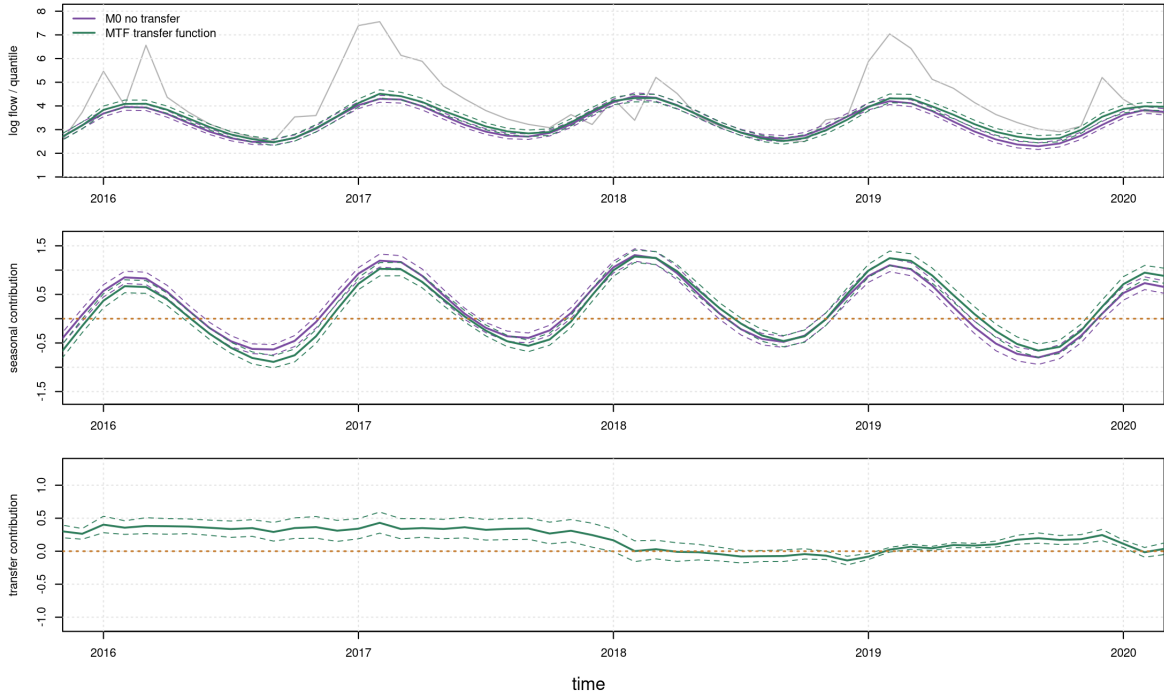
Figure 6: Example 3: Big Tree water flow. Top: MAP estimates and 95% CrIs of the fitted 0.15 quantile from the no-transfer baseline M0 (purple) and transfer-function model MTF (green), plotted with the data (grey) from 2016 to 2020. Middle: MAP estimates and 95% CrIs of the combined seasonal components implied by the annual, semiannual, and low-frequency harmonics. Bottom: MAP estimates and 95% CrIs of the transfer-function contribution from NOI and AMO in MTF. The horizontal orange dotted lines are at zero for reference.
