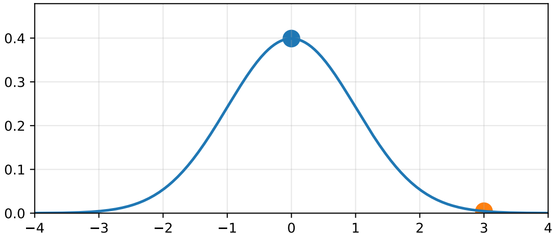
Log-Likelihood Score
