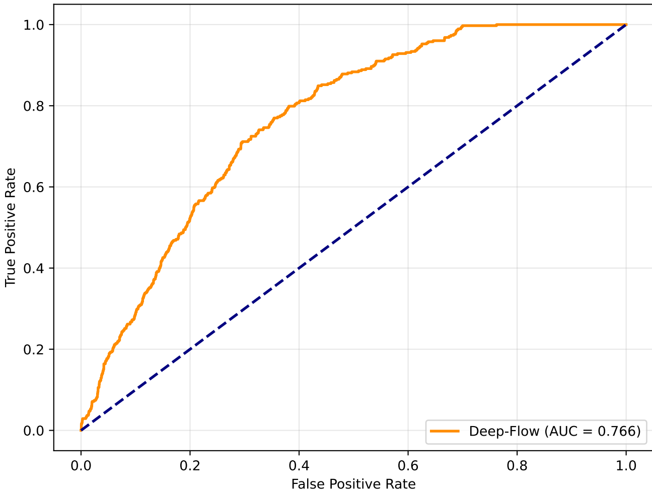
ROC Curve: Detecting Safety Critical Events
