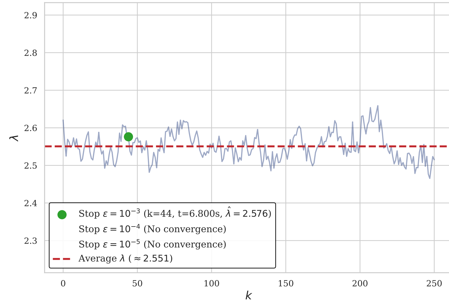
M = 250 (Time/Iter: 154.5 ms — Total Time: 38.63s )
