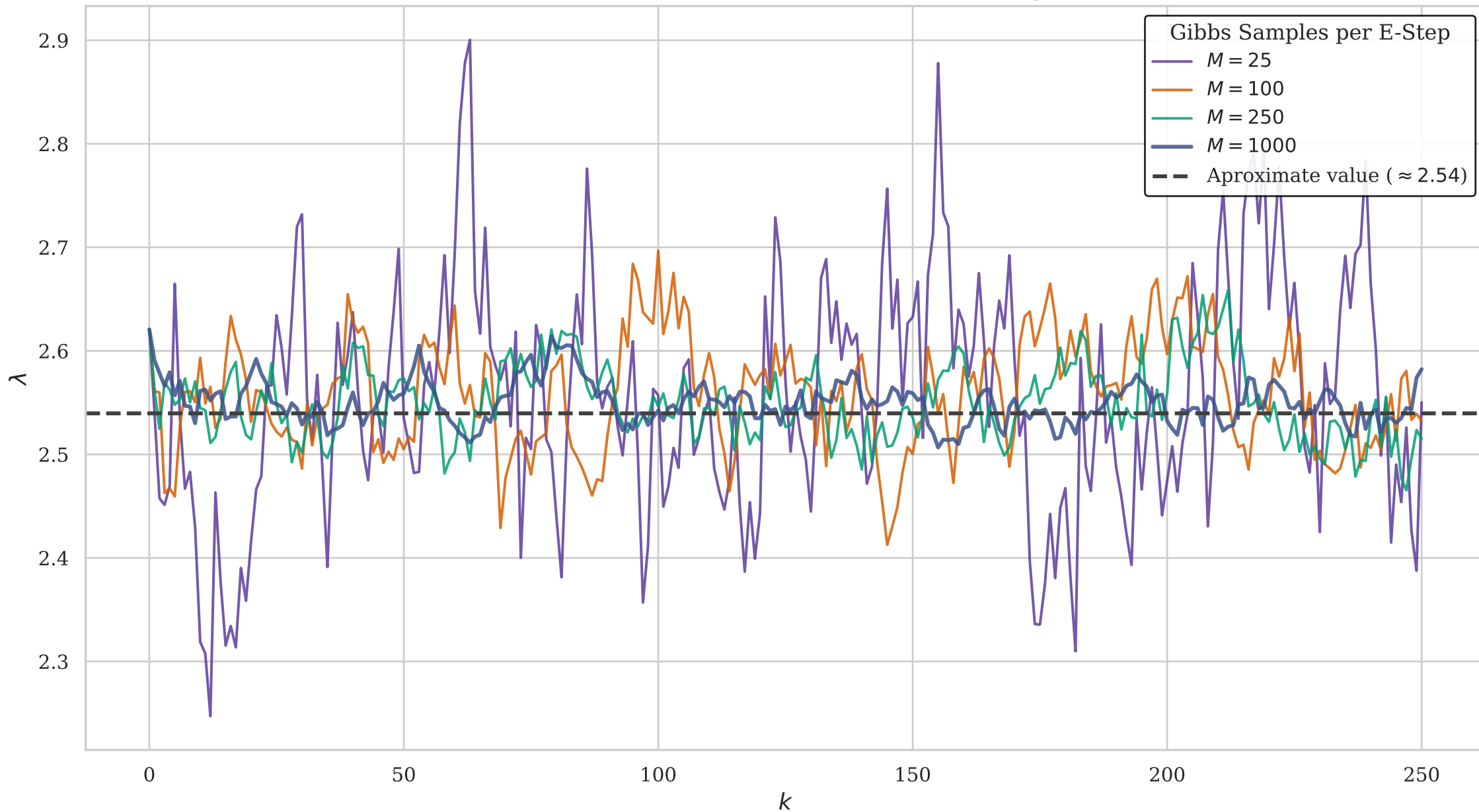
Impact of Sample Size ( M ) on \lambda Convergence
