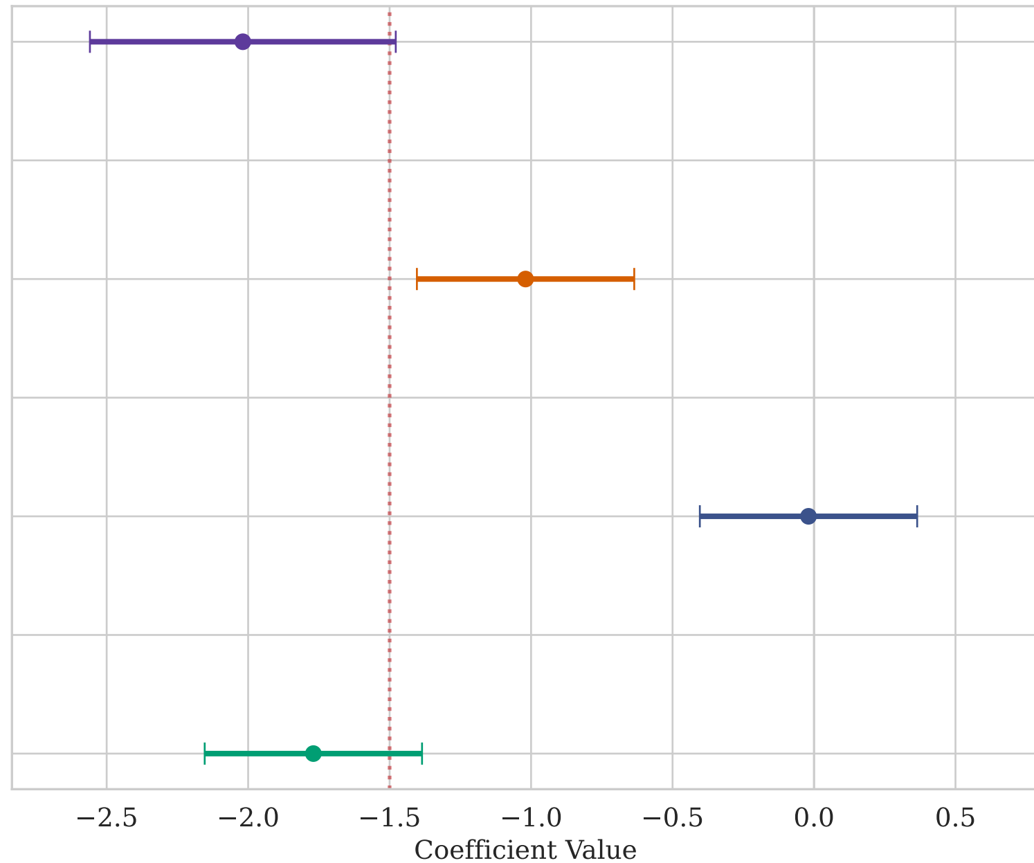
95% Credible Intervals for \beta_3
