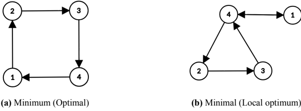
Figure 2. Comparison of reduction outcomes. (a) The optimal Hamiltonian cycle (4 edges). (b) A minimal equivalent graph (5 edges) resulting from premature edge deletion by the greedy approach.
