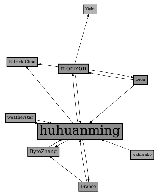
Random Walk Community (tr) 2 Community Quality = 0.0203076923076923
