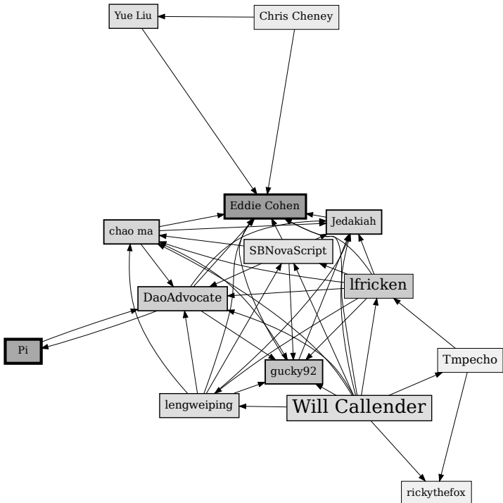
Spin Glass Community 1 Community Quality = 0.738812785388128
