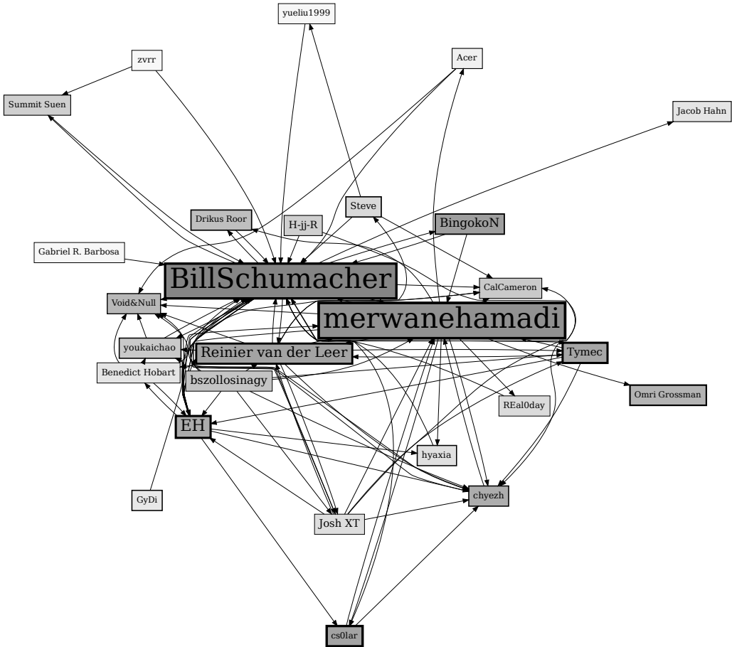
Spin Glass Community 3 Community Quality = 0.399968592964824
