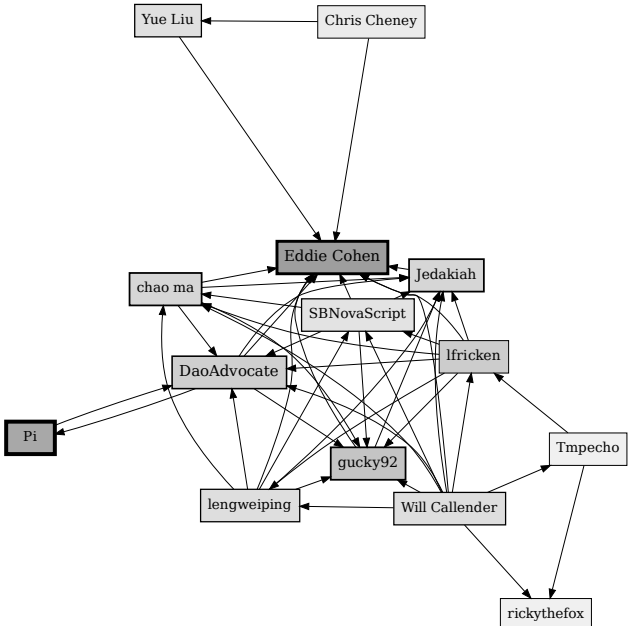
Spin Glass Community (tr) 1 Community Quality = 0.738812785388128
