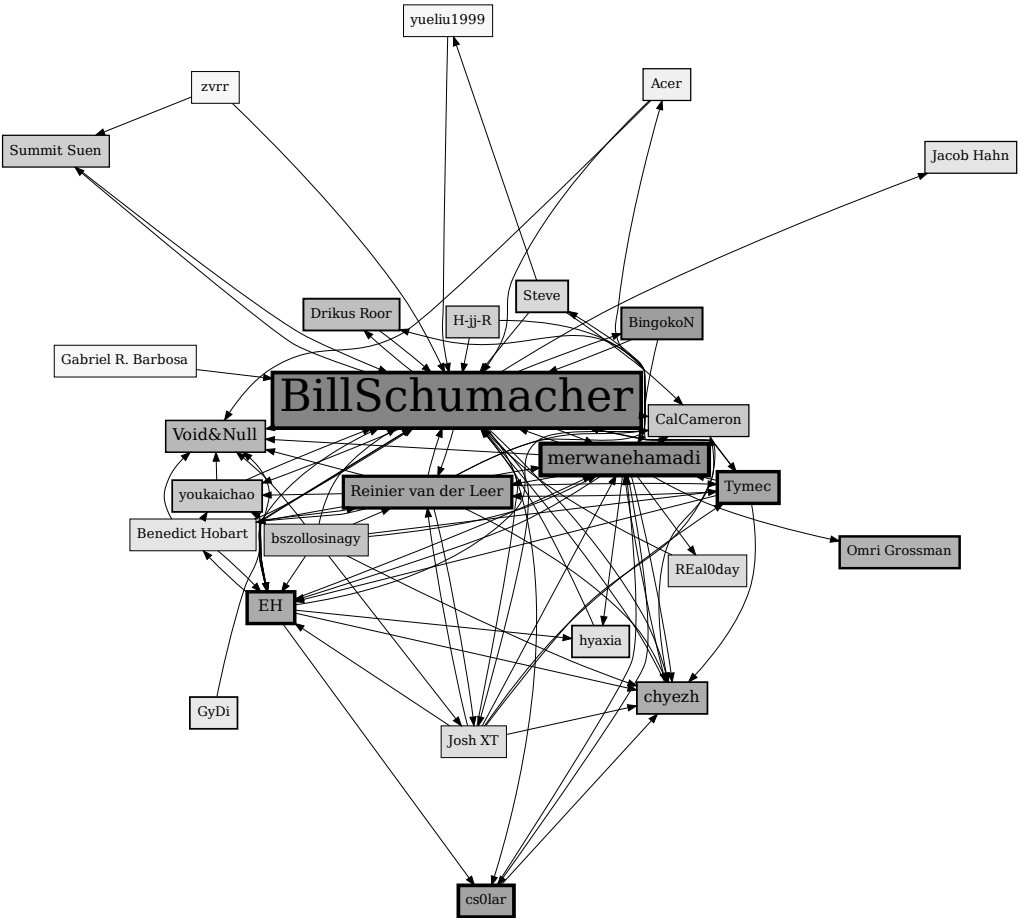
Spin Glass Community (tr) 3 Community Quality = 0.399968592964824
