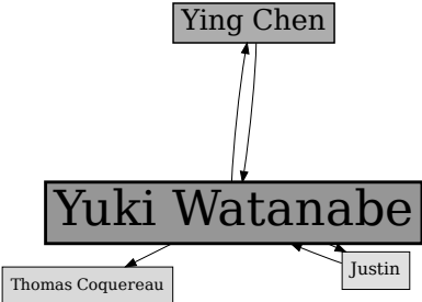
Spin Glass Community 4 Community Quality = 0.352631578947368
