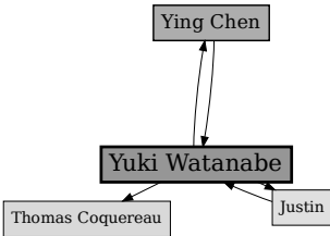
Spin Glass Community (tr) 4 Community Quality = 0.352631578947368
