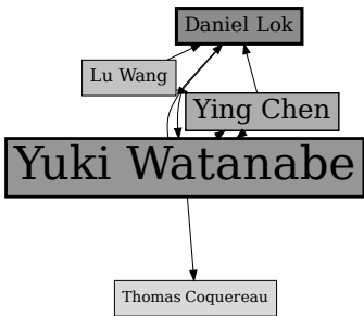
Random Walk Community 3 Community Quality = 0.275275735294118
