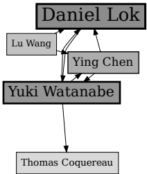
Random Walk Community (tr) 3 Community Quality = 0.275275735294118
