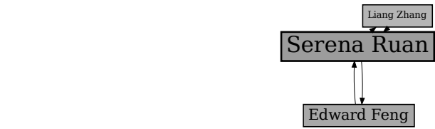
Random Walk Community (tr) 2 Community Quality = 0.164218958611482
