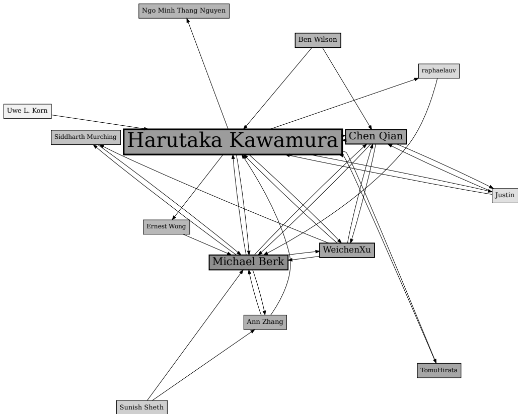
Random Walk Community 1 Community Quality = 0.256936736958935
