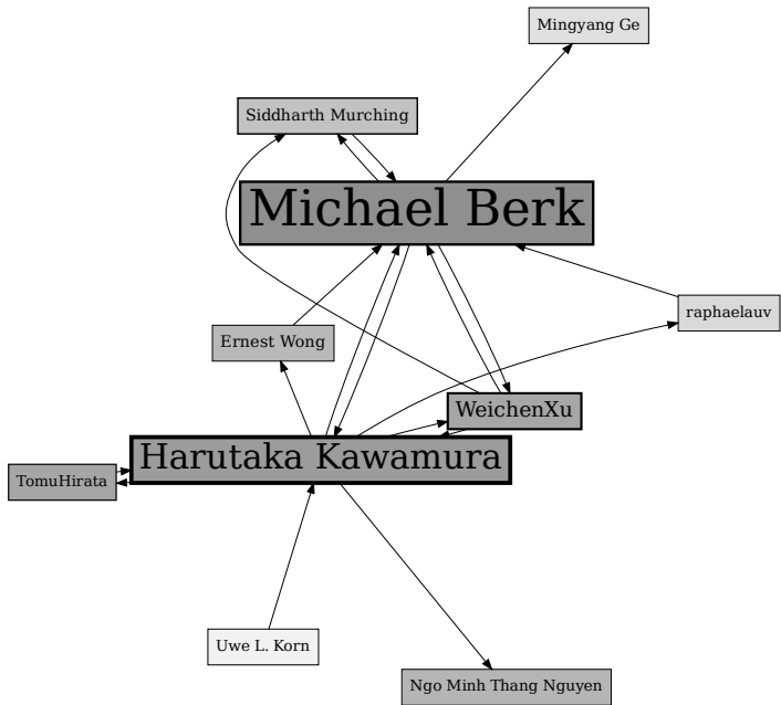
Spin Glass Community (tr) 1 Community Quality = 0.454718055819252
