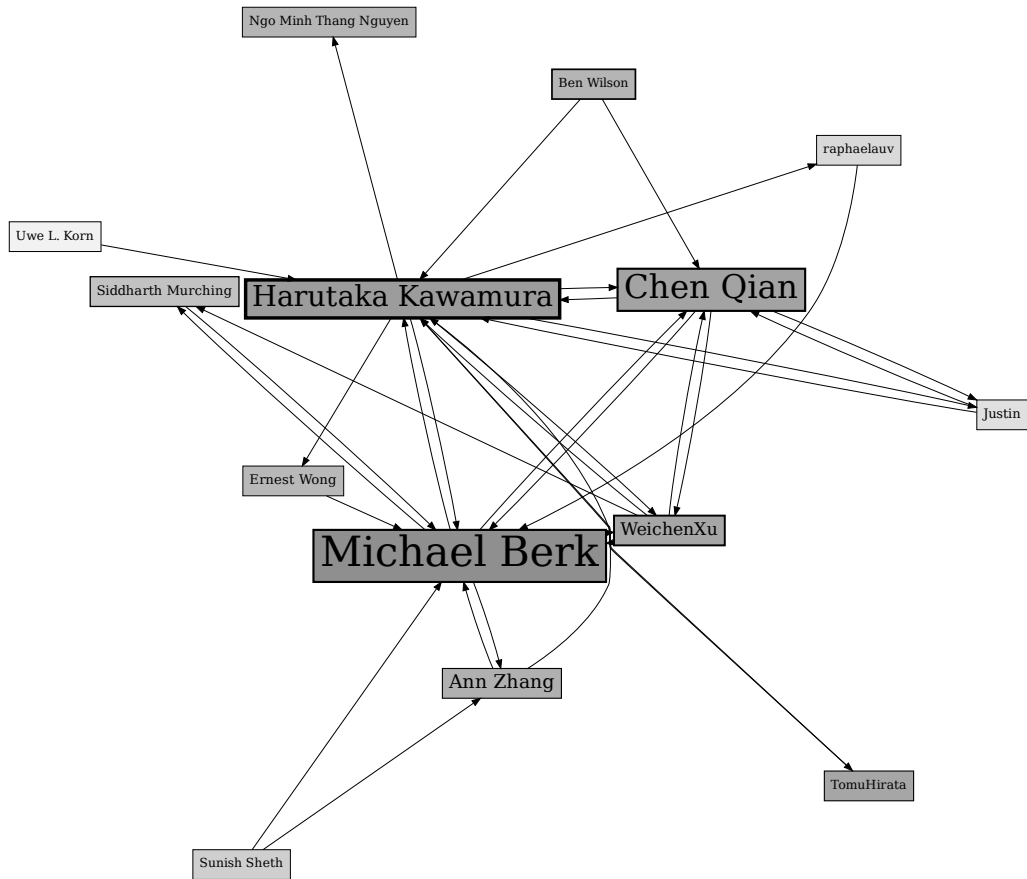
Random Walk Community (tr) 1 Community Quality = 0.256936736958935
