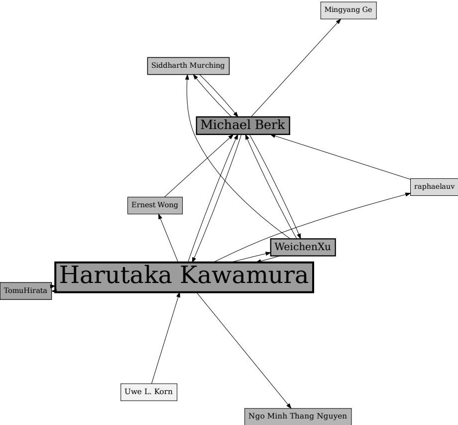
Spin Glass Community 1 Community Quality = 0.454718055819252
