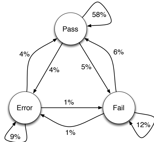
Figure 2: Summary of the transitions between build states in our dataset. Each transition is caused by one or more commits. Pass→Pass persisted for an average of 5.6 builds, Error→Error persisted for 2.6 builds, while Fail→Fail persisted for 2.9 builds.
