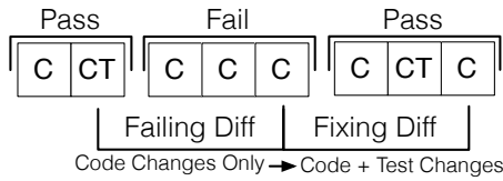
Figure 3: As developers work on their systems their commits often change the state of the build. Each box represents a commit; builds are often not run on every commit but instead on blocks of commits. A C label on a commit means the code under test was changed; a T label means the test code was changed. The figure shows a failure caused by a code change that was resolved by changing both code and test files.
