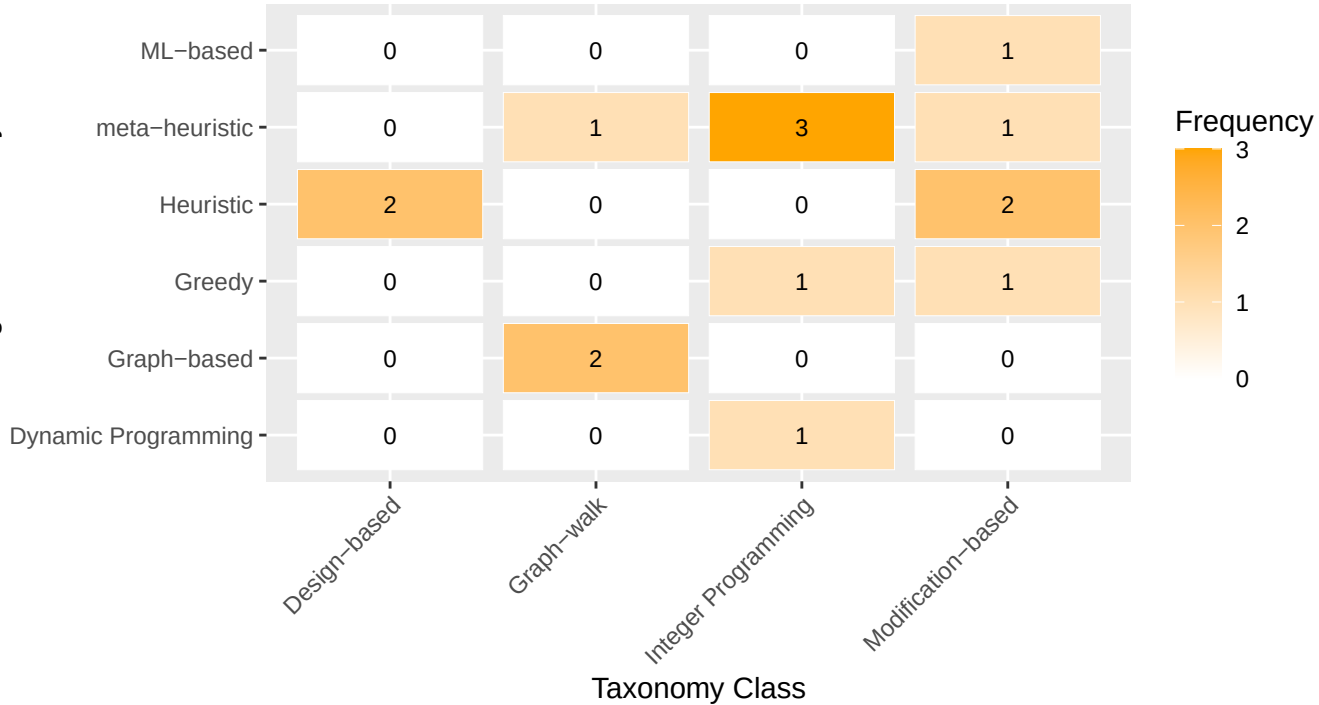
Algorithmic Family
