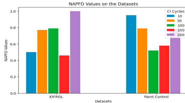
Figure 5: NAPFD values on different CI Cycles
