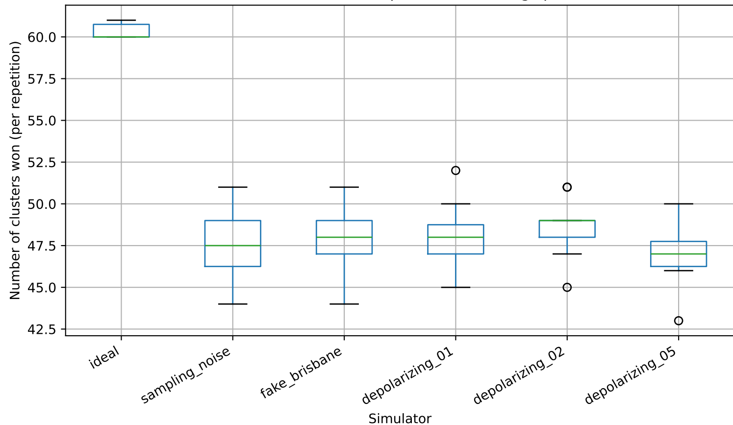
Cluster-level wins per simulator — gzip
