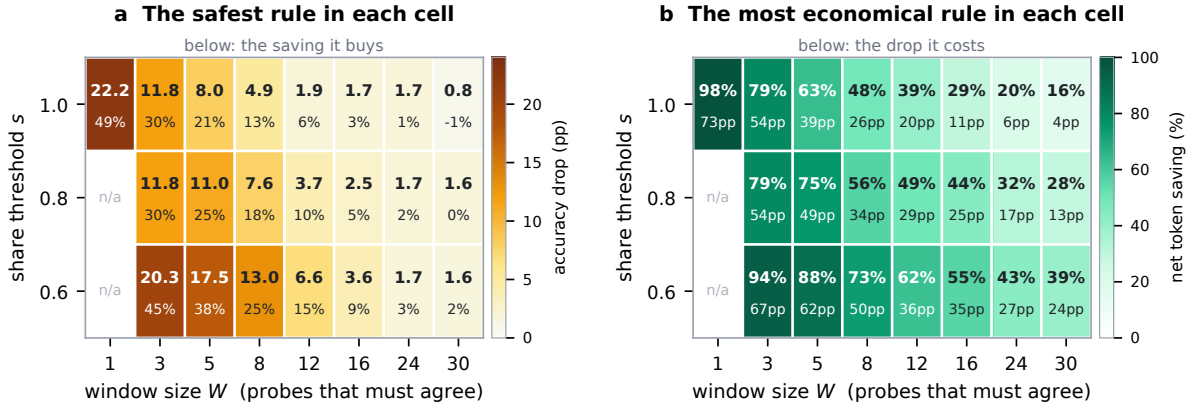
Figure 5: The safe-and-saving corner is empty across the entire rule space. Dev split, macro-averaged over the 18 environments. Each cell holds the 160 rules sharing its (W, s) , summarised by the two members a gate interrogates: (a) the cell’s safest rule (colour: accuracy drop; number: the saving it buys) and (b) its most economical rule (colour: net saving; number: the drop it costs). A cell would be outlined in green if any of its rules cleared the conservative gate (drop \leq 1.0 pp and saving \geq 10\% ); none is.
