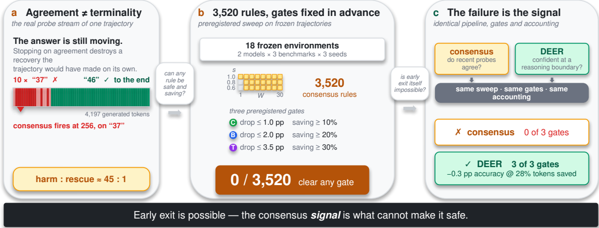
Figure 1: The argument in one picture. (a) On MATH500 problem 68 (DeepSeek-R1-Distill-Qwen-7B, dense 64-token probes) the model emits the same wrong answer, 37, for ten consecutive probes; a three-probe rule fires at token 256 and commits it. Left to run, the trajectory reaches the correct 46. Ribbon colours: red the dominant wrong answer, pink other wrong answers, green correct. (b) The preregistered sweep of 3,520 rules, replayed on 18 frozen environments against three gates fixed in advance. None clears any gate. (c) Swept through the same pipeline, gates and accounting, a boundary-confidence method (DEER) clears all three—on the test split, at 4\times scale and on a different architecture too (§5.5).
