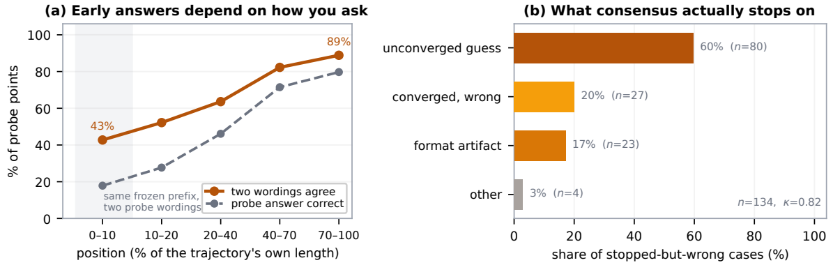
Figure 2: Two sides of the stability-terminality gap. (a) The same frozen prefix (DeepSeek-R1-Distill-Qwen-7B, MATH500) re-probed with two differently worded answer queries. Early in a trajectory the two wordings return the same current answer less than half the time (43% in the first tenth) and the probed answer is usually wrong; by the end they nearly always coincide (89%) and are usually correct. Position is a fraction of each trajectory’s own length. (b) All 134 stopped-but-wrong cases, labelled independently by two annotators ( \kappa=0.82 ): three in five commit to an answer the model had not converged on, one in six to a probe-format artifact, fewer than one in five to a genuinely settled wrong value.
