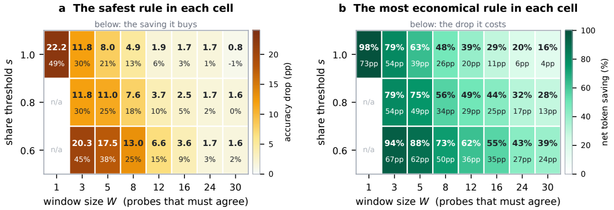
Figure 5: The safe-and-saving corner is empty across the entire rule space. Dev split, macro-averaged over the 18 environments. Each cell holds the 160 rules that share its (W, s) and differ only in the operational knobs, summarised by the two members a gate interrogates. (a) the cell’s safest rule: colour is its accuracy drop and the number beneath is the saving that rule buys. Larger windows and stricter thresholds do drive the drop towards the 1.0 pp cap—but the saving falls with it, reaching −1% at W=30, s=1.0 . (b) the cell’s most economical rule: colour is its net saving and the number beneath is the drop it costs. Substantial saving is available everywhere, at 4–73 pp. A cell would be outlined in green if any of its rules cleared the conservative gate (drop \leq 1.0 pp and saving \geq 10\% ); none is.
