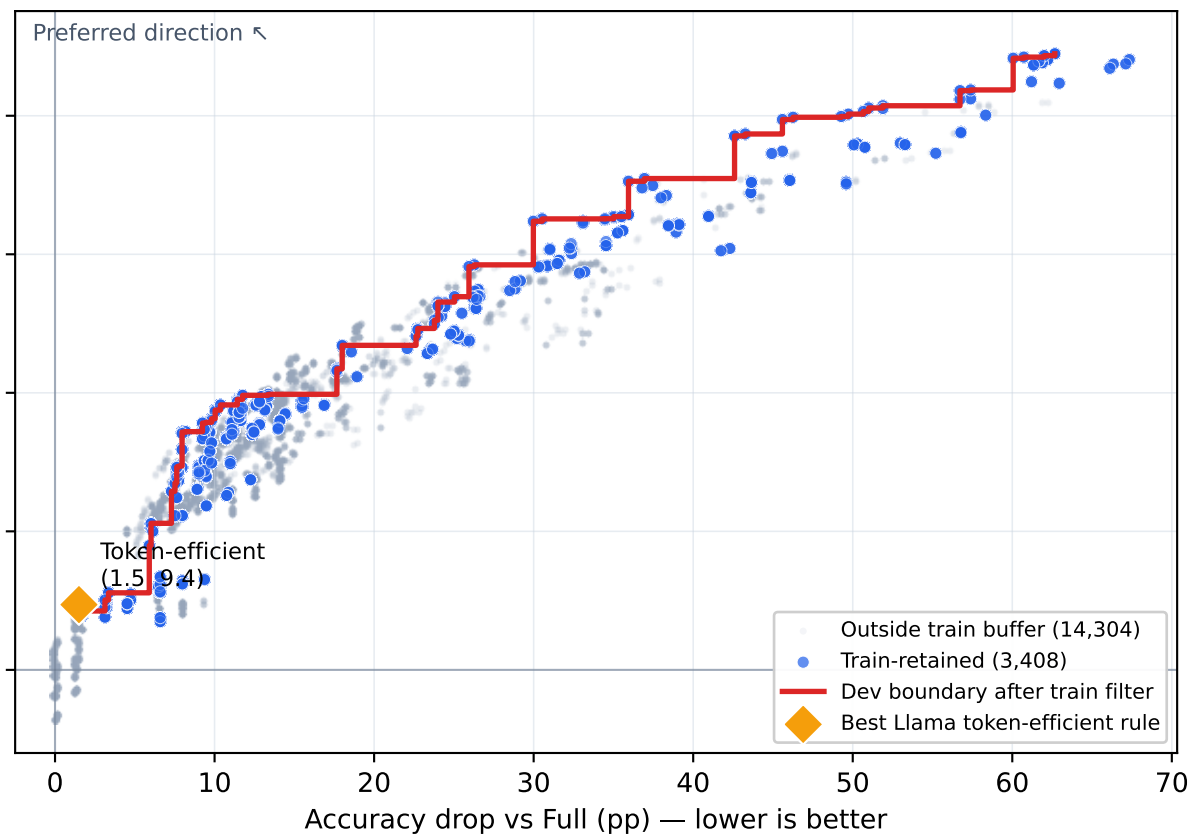
Dev: transfer of train-retained rules
