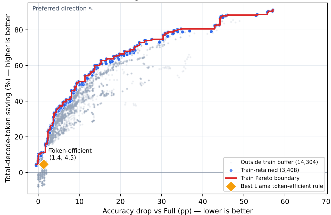
Train: near-Pareto filtering
